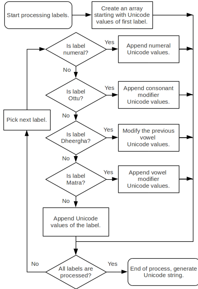
Figure 4.10: The flowchart of Kannada labels to Unicode conversion. The four important sections in the flowchart check the different combinations of previous and present labels that modify the generated Unicode sequence.
