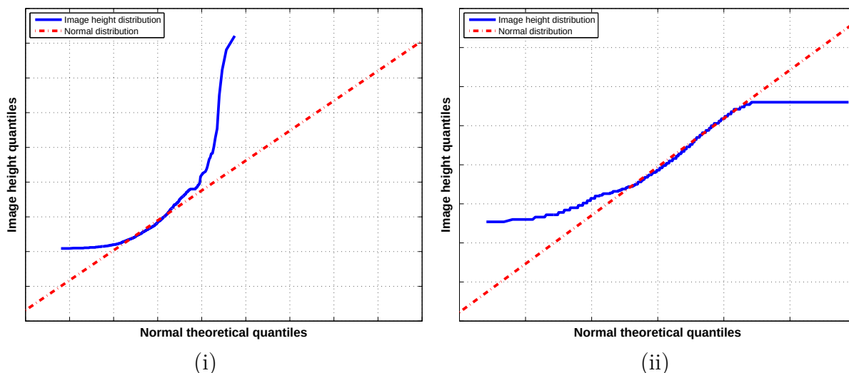
Figure 3.11: Q-Q plots of image heights for ICDAR 2011 data set. The actual image height quantiles are plotted against the normal theoretical quantiles. (i) Before height normalization of images. (ii) After height normalization of images.
