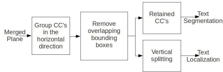
Figure 2.9: The final section of the OTCYMIST method which segments and localizes the text. Vertical splitting block locates the individual words from a group of words.
