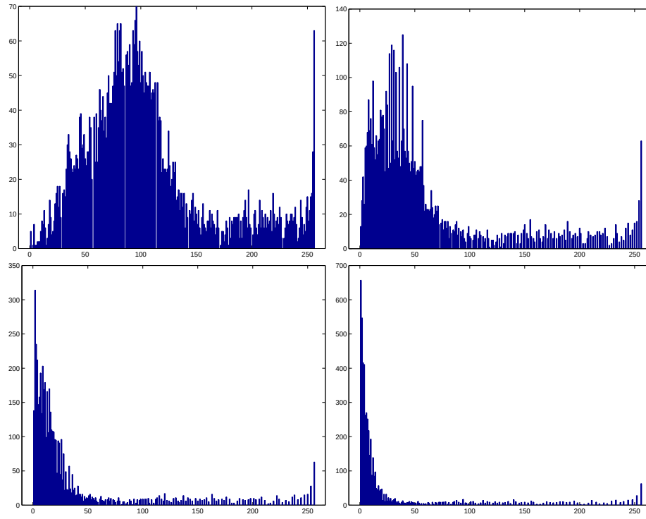
Figure 3.3: Histogram plots obtained for the sample word image ‘Ticket,’ shown in Fig. 3.2 after power-law transformation with \gamma = 1, 2, 3 and 4, respectively. The modified pixel values change the histogram significantly.
