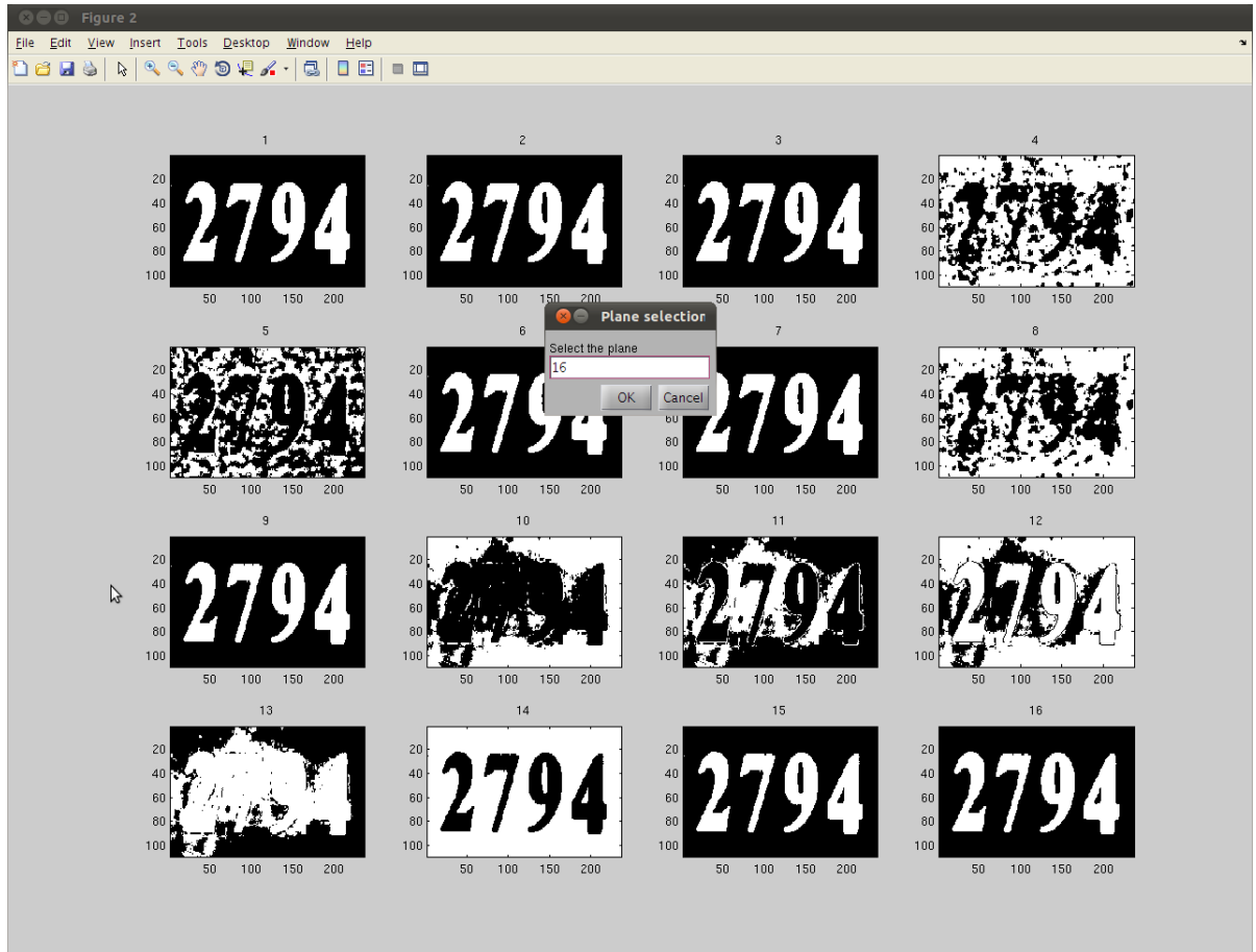
Figure A.3: Automated segmentation by MAST. Sixteen distinct segmentation results generated by MAST for a chosen scene word image shown in Figure A.1. The user selects the best result using a keyboard input (shown in the middle).
