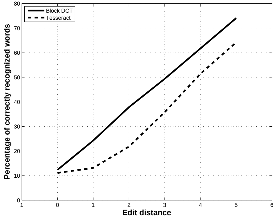
Figure 4.12: Plot of word recognition versus edit distance for Tesseract OCR and our classifier using block DCT OCR for manually segmented word images (Benchmark images). For values of the edit distance of one and more, the gap between the two recognizers is more than 10%.
