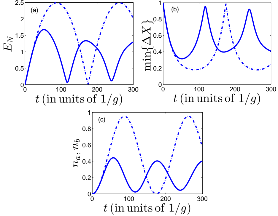
Figure 3.1: (a) Logarithmic negativity E_N in (3.4) is evaluated as a function of time t (in units of 1/g ), in the absence of dissipations. The solid lines are evaluated numerically by solving the Schrödinger equation of motion using the Hamiltonian (3.7), according to the App. D, whereby the dash-dotted lines are the corresponding results for \chi = 0 . The corresponding plots for the minimum variance of a composite quadrature \min\{\Delta X(\theta_a, \theta_b)\} (see Eq. (3.13)) with respect to the angles \theta_a and \theta_b , are shown in panel (b). The value of \Delta X = 1 corresponds to the shot-noise limit. The curves in (c) display the field modes population n_a = \langle a^\dagger a \rangle and n_b = \langle b_Q^\dagger b_Q \rangle as a function of time in which the two curves for n_a and n_b are superimposed. The parameters are \omega_z = 100g, \Omega = 5g, N = 50, \delta_c = -100.55g and the decay rates \kappa and \Gamma are set to zero. Here \delta_b = 100.5g . The oscillatory behaviour for the curves is due to non-resonance condition \delta_c \neq -\delta_b (see App. C). The initial state is the vacuum for both modes.
