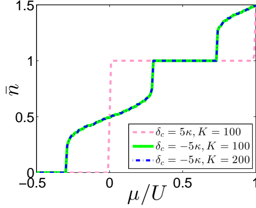
Figure 4.5: Mean density \bar{n} as a function of the chemical \mu (in units of U ) at t = 0 in a one-dimensional lattice. The curves have been obtained by a diagonalization of Hamiltonian (4.41) for (dashed line) \delta_c = 5\kappa and (solid line) \delta_c = -5\kappa , both for K = 100 . The diagonalization, is based on the iterative calculation of the evaluating the value of \hat{\Phi} , which has been treated in a mean-field way, i.e., \hat{\Phi}^2 \approx \langle \hat{\Phi}^2 \rangle + 2\langle \hat{\Phi} \rangle \hat{\Phi} . The other parameters are s_0 = 0.006\kappa (with \kappa = 2\pi \times 1.3 MHz), u_0 = 0.8\kappa , and U/\hbar = 50 Hz. Here, the chemical potential is reported without the constant shift \epsilon^{(0)} , \mu \rightarrow \mu - \epsilon^{(0)} . The dash-dotted line has been evaluated for the same parameters of the solid line, except with K = 200 . It shows that the results remain invariant as the system size is scaled up.
