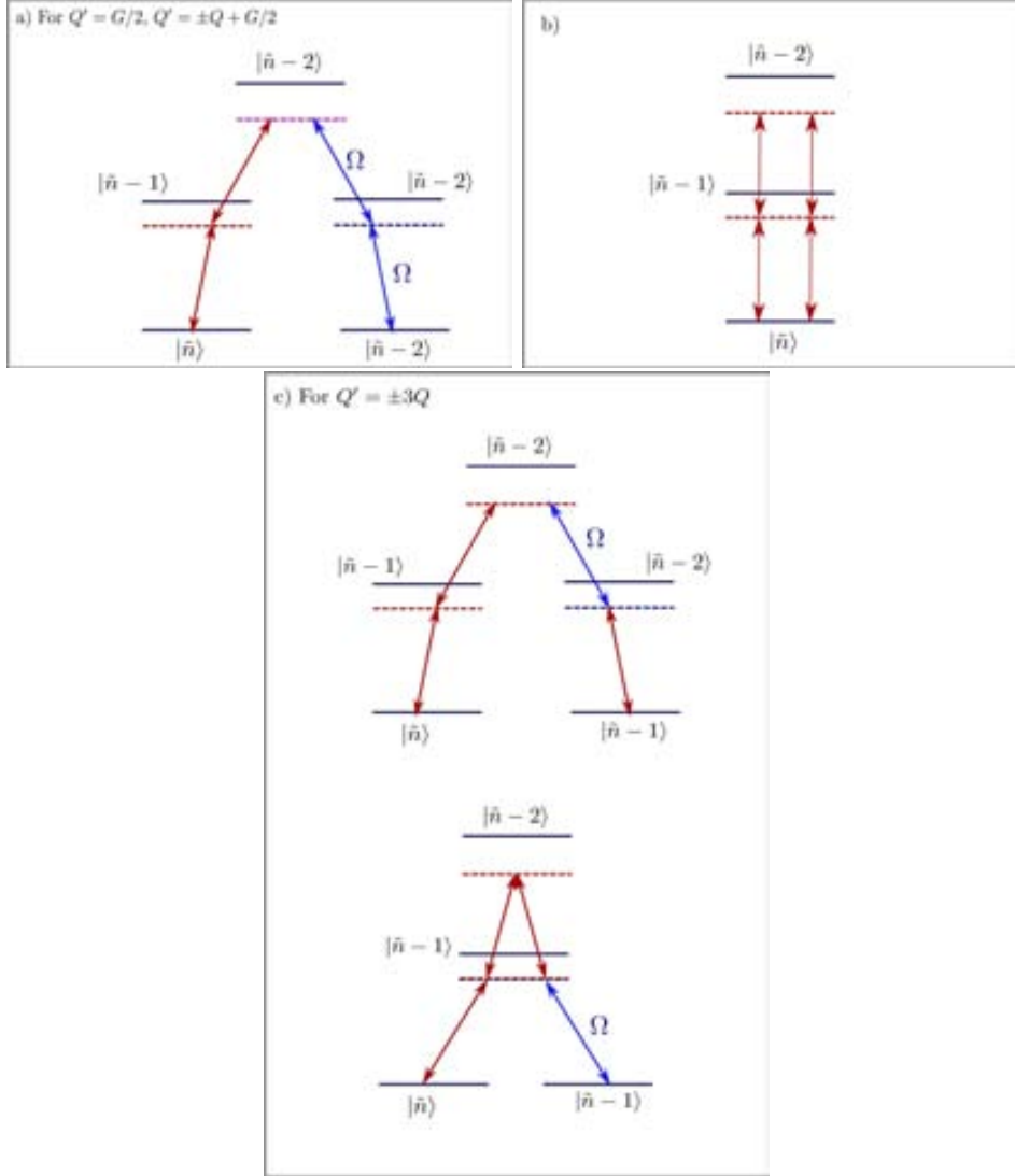
Figure 2.3: Schematic diagram of transitions which fulfill the phase-matching condition till fourth order. State |\tilde{n}\rangle denote the number state of the polariton mode \gamma_1 . The blue arrows denote the laser-induced couplings and the red arrows denote the creation (annihilation) of polaritons due to the coupling with the cavity field. See text for a detailed discussion.
