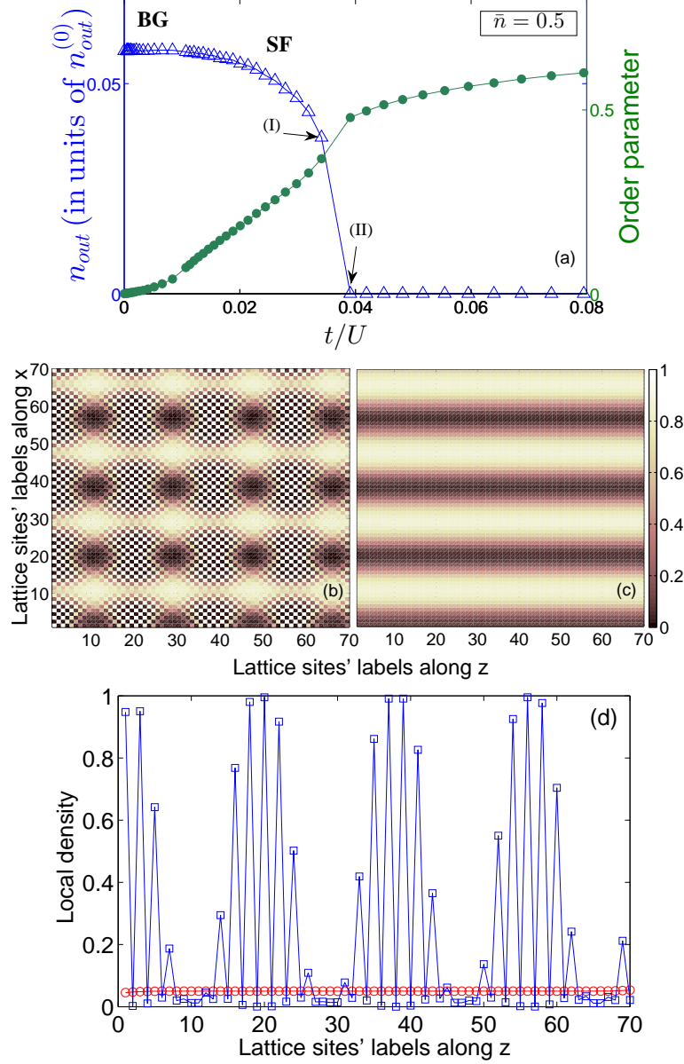
Figure 4.12: (a) Intensity at the cavity output, n_{\text{out}} = \langle \hat{a}_{\text{out}}^\dagger \hat{a}_{\text{out}} \rangle as a function of t (in units of U ) for the parameters of Fig. 4.11(a) and by fixing \bar{n} = 0.5 . Here, n_{\text{out}} is in units of n_{\text{out}}^{(0)} = \kappa n_{\text{cav}}^{(\text{max})} where n_{\text{cav}}^{(\text{max})} = s_0^2 K / (\hat{\delta}_{\text{eff}}^2 + \kappa^2) is the maximum number of intracavity photons, obtained when all atoms scatter in phase into the cavity mode. The curve with circles (right y -axis) gives the corresponding order parameter. Subplot (b) displays the contour plot of the local density distributions at point (I) in panel (a), where t = 0.034U , \mu = 0.106U , \langle \hat{\Phi} \rangle = 0.136 . Subplot (c) displays the local density distributions at point (II) in panel (a), where t = 0.039U , \mu = 0.122U , while \langle \hat{\Phi} \rangle \simeq 0 . Subplot (d) displays the local density \langle \hat{n}_{i,j} \rangle as a function of the site numbers along z for the lattice site 20 along x . The blue squares (red circles) correspond to the parameters of panel (b) (panel (c), respectively).
