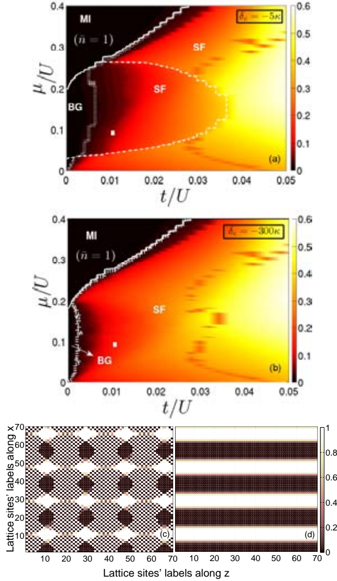
Figure 4.11: (a), (b) Order parameters in \mu - t plane (in units of U ) obtained by the mean-field calculation for a 70 \times 70 lattice with periodic boundary conditions. The dotted lines separate the region with vanishing order parameters, while the solid line identifies the border for the incompressible MI state at density \bar{n} . The regions with finite compressibility and vanishing order parameters correspond to BG phases. The dashed line separates the region where the photon number is 2 order of magnitude larger than outside. The parameters are s_0 = 0.15\kappa , u_0 = 237\kappa , \Delta_a = 2\pi \times 58 GHz, whereas (a) \delta_c = -5\kappa and (b) \delta_c = -300\kappa . In the latter case the effect of the cavity potential is expected to be small. The local densities \langle \hat{n}_{i,j} \rangle of the phase diagram at \mu = 0.092U and t = 0.01\kappa are shown in (c) for \delta_c = -5\kappa and \bar{n} = 0.5 (squared point in (a)) and in (d) for \delta_c = -300\kappa and \bar{n} = 0.446 (squared point in (b)).
