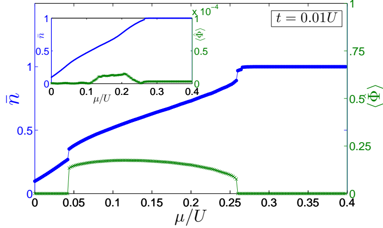
Figure 4.10: Mean density \bar{n} (blue line) and \langle\Phi\rangle (green line with crosses) versus \mu (in units of U ) for a two-dimensional lattice. The curves are evaluated using local mean-field for t = 0.01U and K = 70 \times 70 . The parameters are \Delta_a = 2\pi \times 58\text{GHz} , s_0 = 0.15\kappa , \delta_c = -5\kappa , u_0 = 237\kappa ( \kappa = 2\pi \times 1.3\text{MHz} ). Inset: Same curves but for \delta_c = -300\kappa . Note that the maximum value of \langle\Phi\rangle is 3 orders of magnitude smaller than for \delta_c = -5\kappa .
