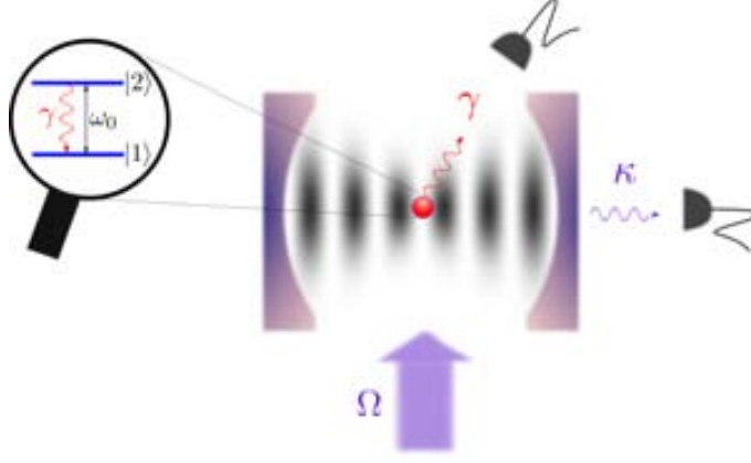
Figure 1.1: Schematic picture of an atom inside a Fabry-Pérot cavity, which is driven by a transverse laser field at Rabi frequency \Omega . The wiggled lines symbolize cavity decay at rate \kappa and spontaneous emission at rate \gamma , with which photons are emitted outside of the system. The inset shows a sketch of the internal degrees of freedom of the atom, where ground and excited state of the atoms are denoted by |1\rangle and |2\rangle , respectively, while \omega_0 is the atomic transition frequency. Here we assume that one of the cavity mirrors (left mirror) has zero transmittivity.
