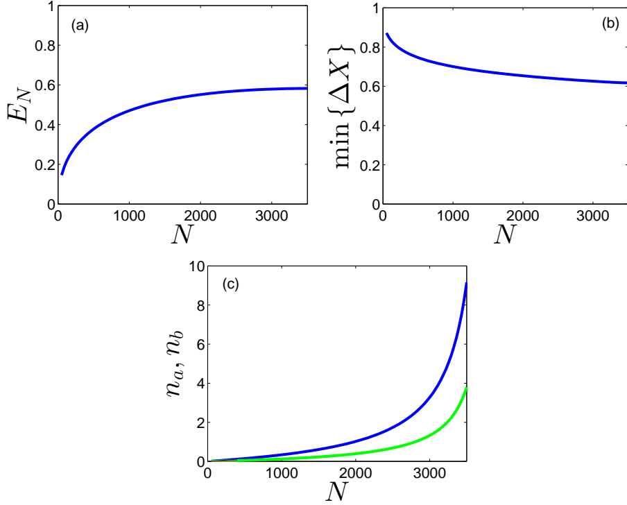
Figure 3.9: The same plots as in Fig. 3.6, as a function of the number of atoms N for \kappa = 2.5g and \Gamma = 7.5g . In (c) the dark blue lines represent n_a and the light green lines represent n_b .
