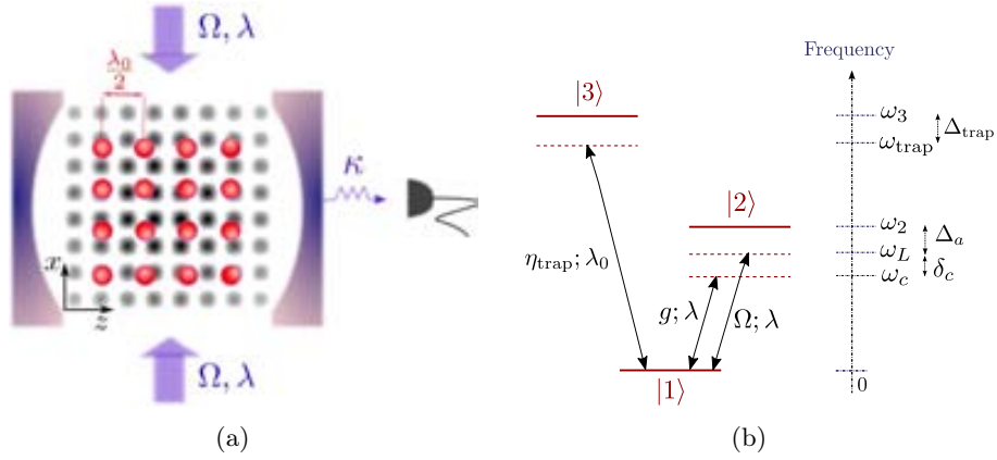
Figure 4.4: (a) Ultracold atoms are tightly confined by an optical lattice of periodicity \lambda_0/2 . They are driven by a weak transverse laser at Rabi frequency \Omega and strongly coupled to the mode of a standing-wave cavity both at wavelength \lambda . The level structure of the atoms is shown in panel (b) where the transition between internal levels |1\rangle and |2\rangle is driven by the transverse laser which is close to resonance with the cavity mode, while the optical lattice field whose depth is determined by an amplitude \eta_{\text{trap}} is close to resonance with the atomic transition |1\rangle \rightarrow |3\rangle . Since \lambda and \lambda_0 are incommensurate, one would expect no coherent scattering into the cavity mode. The mechanical effects due to multiphoton scattering, however, give rise to an incommensurate quantum potential, which mediates an effective long-range interaction between the atoms and modifies the properties of the quantum ground state. As a result, the intracavity photon number can be large. The corresponding ground state can show features typical of a BG.
