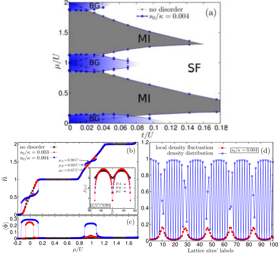
Figure 4.8: Results of QMC simulations for a one-dimensional lattice ( \beta \gg 1 ) with 100 sites and periodic boundary conditions. (a) The phase diagram is obtained by QMC calculation for a one-dimensional lattice with 100 sites for s_0 = 0.004\kappa . The results are compared with the pure case (dotted curves). (b) Linear density \bar{n} and (c) \langle \hat{\Phi} \rangle as a function of \mu for t = 0.053U and s_0/\kappa = 0.003 (triangles), s_0/\kappa = 0.004 (circles), and s_0 = 0 (squares): The number of photons is different from zero for the parameters corresponding to the blue regions in (a). The inset of (b) displays the Fourier transform of the pseudo current-current correlation function J(\omega) [141–143] for the parameters indicated by the arrows in the curve of (b): the extrapolated value at zero frequency is proportional to the SF density. (d) Local density distribution \langle \hat{n}_i \rangle (empty points joined by the blue curve) and local density fluctuations \langle \hat{n}_i^2 \rangle - \langle \hat{n}_i \rangle^2 (filled points joined by the red curve) as a function of the site for \mu = 0 and s_0 = 0.004\kappa . The other parameters are as in Fig. 4.5.
