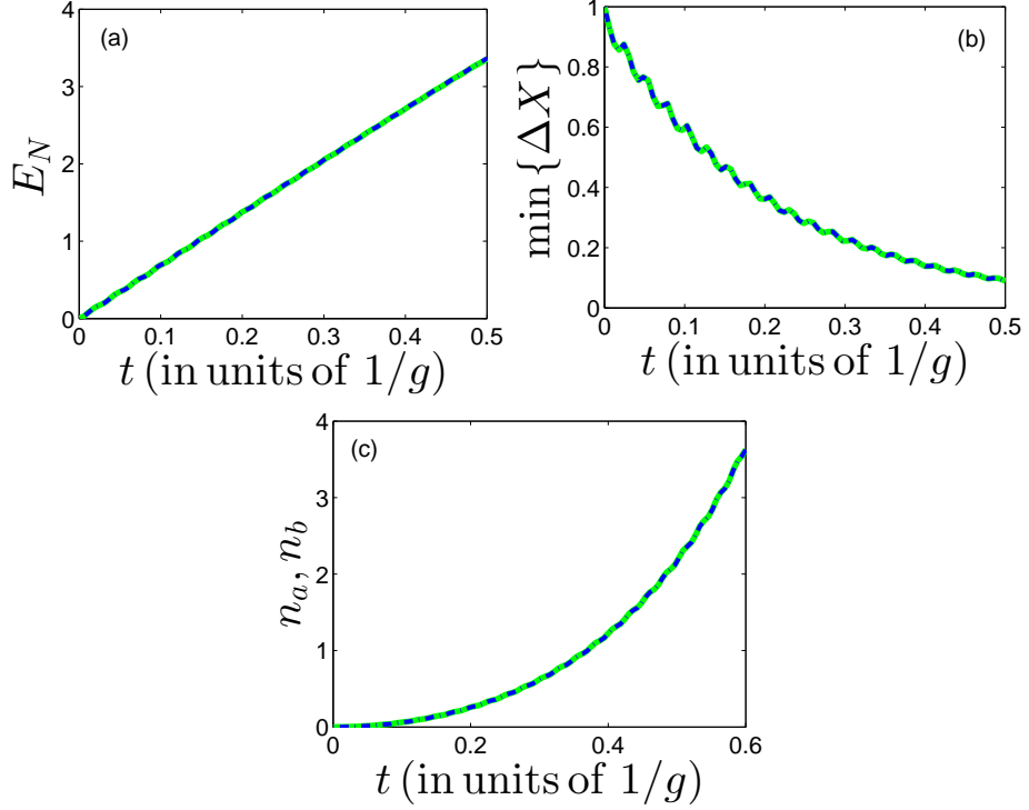
Figure 3.5: The same plots as in Fig. 3.3 with \delta_c = -120g . The populations increase in a smaller time-scale than Fig. 3.4.
