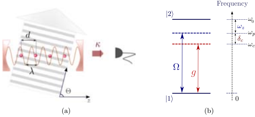
Figure 1.2: (a) A periodic array of atoms, with interparticle distance d , is confined along the axis of a standing-wave optical cavity at frequency \omega_c and is transversally driven by a laser, whose wave vector forms the angle \Theta with the cavity axis. The atomic internal transition and the relevant frequency scales are given in (b), with |1\rangle and |2\rangle ground and excited state of an optical transition with frequency \omega_0 and natural linewidth \gamma . The frequencies \omega_z = \omega_0 - \omega_p and \delta_c = \omega_c - \omega_p denote the detunings between the laser frequency \omega_p and the atomic and cavity frequency, respectively. The other parameters are the laser Rabi frequency \Omega , the atom-cavity coupling strength g , and the decay rate \kappa of the optical cavity.
