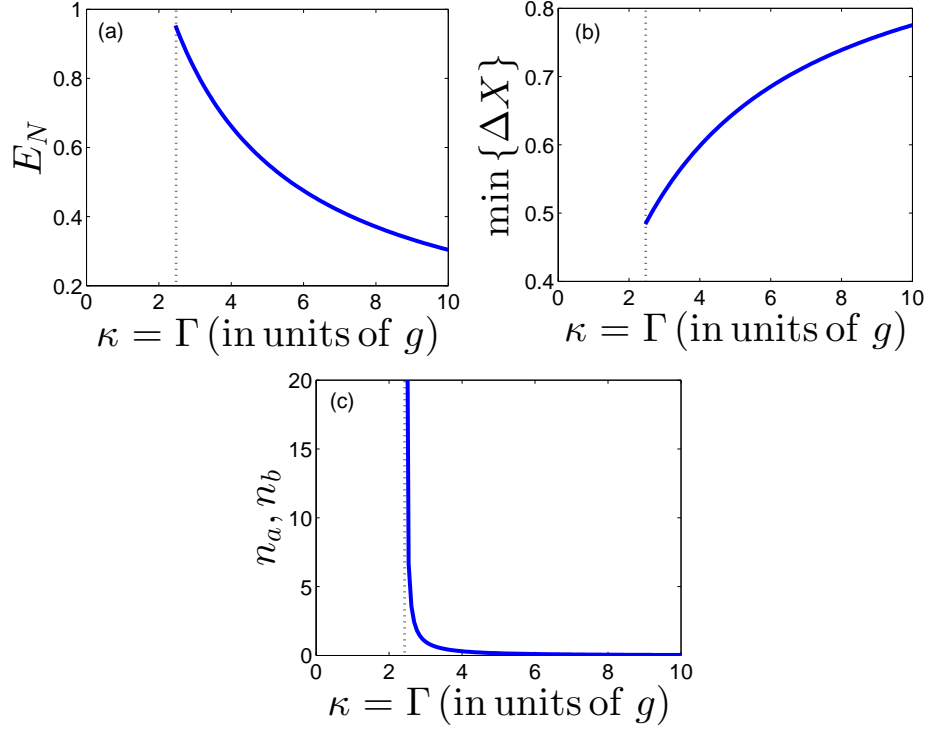
Figure 3.6: (a) Logarithmic negativity E_N is plotted at the steady state as a function of the decay rates \kappa = \Gamma in units of g . In (b) the minimum variance of a composite quadrature \min\{\Delta X(\theta_a, \theta_b)\} (see Eq. (3.13)) with respect to the angles \theta_a and \theta_b at the steady states is evaluated, whereby in (c) the corresponding populations of the field modes n_a = \langle a^\dagger a \rangle and n_b = \langle b_Q^\dagger b_Q \rangle (the two curves are superimposed) are shown as a function the decay rates \kappa = \Gamma (in units of g ). Note that here the two decay rates are varied together. The dotted lines determine the threshold for the steady state. The results are evaluated using the master equation (3.10) with \chi = 0 . The parameters are \omega_z = 100g, \Omega = 30g, N = 1000, \delta_c = -\delta_b = -118g .
