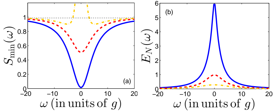
Figure 3.10: (a) Two-mode squeezing spectrum of the emitted fields is evaluated for maximally squeezed composite quadratures \widetilde{\Delta X}^{(\theta_a, \theta_b)} in Eq (3.15) with respect to the angles \theta_a and \theta_b (for details see App. E). (b) Corresponding logarithmic negativity E_N(\omega) as a function of the frequency of the emitted field, is plotted (see App. E). Different curves correspond to the results for the fraction of modes which are detected when the detection efficiencies \eta_a and \eta_b (see App. E) are set to: \eta_a = \eta_b = 1 for the blue solid lines, \eta_a = \eta_b = 0.5 for the red dashed lines and \eta_a = 1 , \eta_b = 0.1 for the yellow dot-dashed lines. The parameters are \kappa = \Gamma = 2.5g , \omega_z = 100g and \delta_c = -\delta_b = -118g and \Omega = 30g , N = 1000 ; \theta_a and \theta_b are set to the values which mainimizes the squeezing spectrum at each frequency \omega . \Delta_a and \Delta_b (see App. E) are set to the frequencies of the normal modes: \Delta_a = -\Delta_b = -121.3g .
