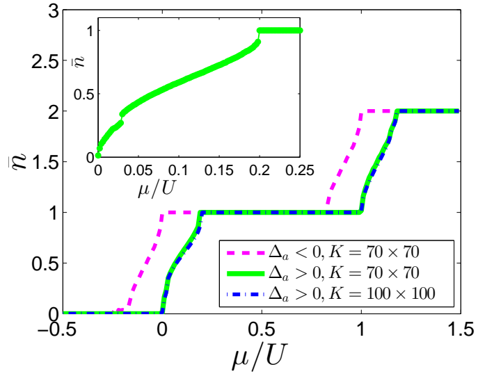
Figure 4.9: Mean density \bar{n} versus \mu (in units of U ) for a two-dimensional lattice. The curves are evaluated by a diagonalization of Hamiltonian (4.39) for t = 0 , in the mean-field approximation when \hat{\Phi}^2 \approx \langle \hat{\Phi}^2 \rangle + 2\langle \hat{\Phi} \rangle \hat{\Phi} , when K = 70 \times 70 and \Delta_a < 0 (dashed line), and K = 70 \times 70 and \Delta_a > 0 (solid line). The parameters are |\Delta_a| = 2\pi \times 58 \text{ GHz} , s_0 = 0.15\kappa , \delta_c = -5\kappa , u_0 = 237\kappa ( \kappa = 2\pi \times 1.3 \text{ MHz} ). Inset: Zoom of the curve at K = 70 \times 70 and \Delta_a > 0 in the compressible phase. The dashed-dotted line for K = 100 \times 100 and \Delta_a > 0 shows, when compared with the solid line, that the qualitative behaviour of the curves remain invariant as the system size is scaled up.
