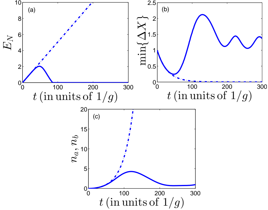
Figure 3.2: The same plots as in Fig. 3.1 with \delta_c = -\delta_b = -100.5g .
