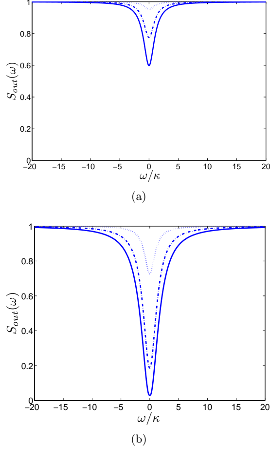
Figure 2.4: Squeezing spectrum for the maximum squeezed quadrature when k = G/2 , Q' = G/2 and Q' \neq Q for \varphi, \phi_L = 0 . The parameters are \Omega = 200\kappa , \omega_z = 10^3\kappa and N = 10, 50, 100 atoms (from top to bottom) for (a) g = 4\kappa and (b) g = 10\kappa . The detuning \delta_c is chosen such that \delta\omega_1 is zero. The curves are evaluated from Eq. (2.49) by numerically calculating the density matrix of the polariton field for a dissipative dynamics, whose coherent term is governed by the effective Hamiltonian in Eq. (2.40). The value g = 4\kappa is consistent with the experimental data of Ref. [86, 87].
