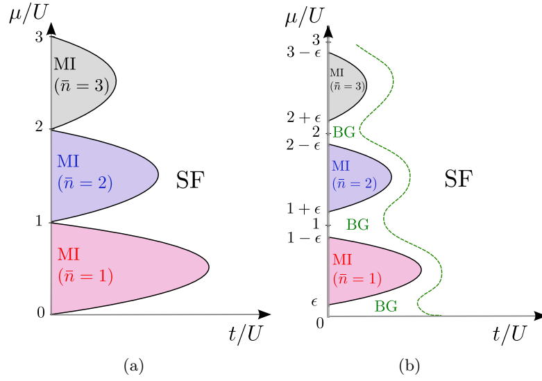
Figure 4.2: Qualitative phase diagram for (a) a pure and (b) a disordered system (with a random disorder) described by the Bose-Hubbard Hamiltonian (4.1). In (a) MI lobes with integer densities \bar{n} = 1, 2, 3 for low values of the tunneling and SF for larger values of tunneling are shown, whereby in (b) the MI-SF transition passes through the BG phase. Here \epsilon = \max |\mu_i|/U which is zero when there is no energy offset at different lattice sites. Solid lines indicate phase transition from MI to compressible phases, and dashed lines separate insulator phases from SF. The phase transition points highly depend on a lattice dimensionality, and a method used to be obtained.
