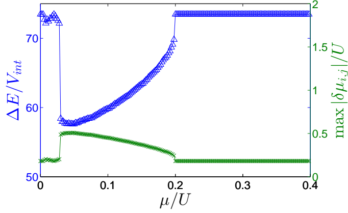
Figure 4.13: Ratio between the energy gap between the two Bloch bands, \Delta E = \sqrt{4E_R|V_0|} , and the interaction energy, V_{\text{int}} = U + \max |\delta\epsilon_{i,j}| , as a function of the chemical potential \mu (in units of U ) and at zero tunneling. The single-band approximation is valid \Delta E/V_{\text{int}} \gg 1 . The green curve with crosses shows the maximum values of \langle \delta\hat{\epsilon}_{i,j} \rangle at the corresponding values of \mu/U . The parameters are as same as in Fig. 4.11(a).
