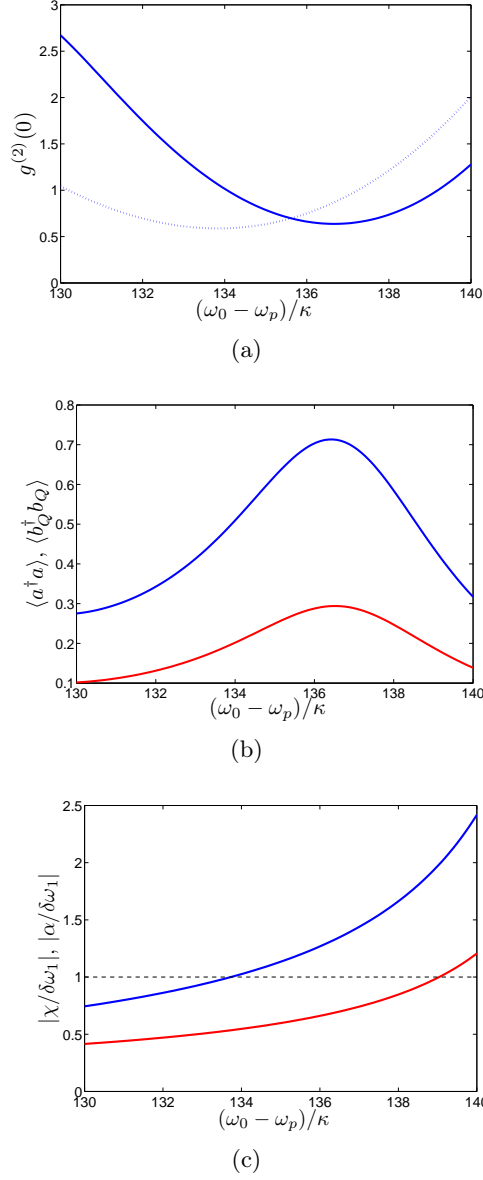
Figure 2.5: (a) Second order correlation function at zero-time delay g^{(2)}(0) versus \omega_p (in units of \kappa ) when the cavity is solely pumped by inelastic processes (here, k = G/2 , Q' \neq Q, 3Q and Q' = G'/2 for \varphi, \phi_L = 0 ). The correlation function is evaluated numerically solving the master equation for the polaritons in presence of cavity decay, with the coherent dynamics given by Hamiltonian (A.1) (solid line) and by Hamiltonian (2.40) (dashed line). (b) Corresponding average number of intracavity photons \langle a^\dagger a \rangle (blue line) and spin wave occupation \langle b_Q^\dagger b_Q \rangle (red line). (c) Ratios |\chi/\delta\omega_1| (blue line) and |\alpha/\delta\omega_1| (red line) versus \omega_p . The parameters are g = 80\kappa , \Omega = 30\kappa , \omega_z - \delta_c = 70\kappa , and N = 2 atoms. At the minimum of g^{(2)}(0) , \omega_z \simeq 137\kappa and \delta_c \simeq 67\kappa .
