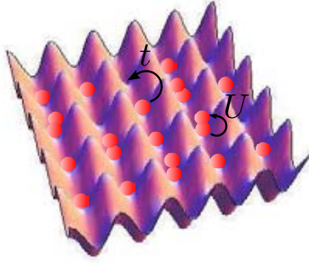
Figure 4.1: Ultracold atoms in a two-dimensional optical lattice which is generated by two counterpropagating laser strongly confined in the third dimension.
