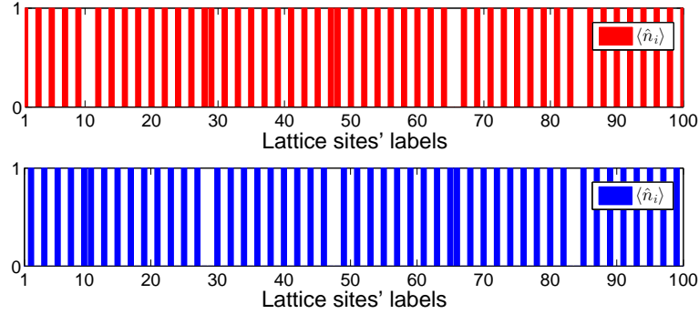
Figure 4.6: Mean density per site, \langle \hat{n}_i \rangle , as a function of the site i for the two distributions corresponding to \delta_c = -5\kappa here for \mu = 0 . The other parameters are the same as in Fig. 4.5. The filled stripes correspond to \langle \hat{n}_i \rangle = 1 , the white stripes to \langle \hat{n}_i \rangle = 0 .
