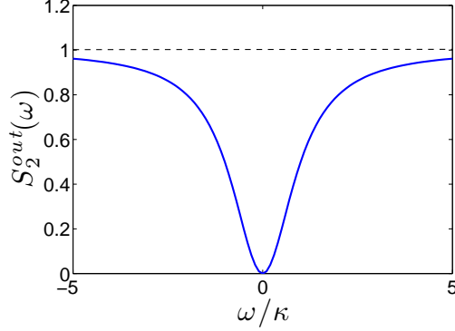
Figure 2.2: The squeezing spectrum S_2^{out}(\omega) at the cavity output related to the quadrature \hat{x}_2^{out} = -i(\hat{a}_{out} + \hat{a}_{out}^\dagger) is plotted at the threshold, i.e. when \alpha = \kappa , in units of the cavity decay rate \kappa . The spectrum is obtained from the Eq. (2.13). The dashed line shows the (classical) shot-noise limit for which S^{out}(\omega) = 1 .
