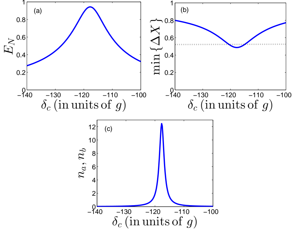
Figure 3.8: The same plots as in Fig. 3.6, as a function of \delta_c (in units of g ) for \kappa = \Gamma = 2.5g . In panel (b), the minimum variance shows more than 50% reduction of the noise, which is due to the single-mode squeezing amplitude \alpha_Q in (3.7).
