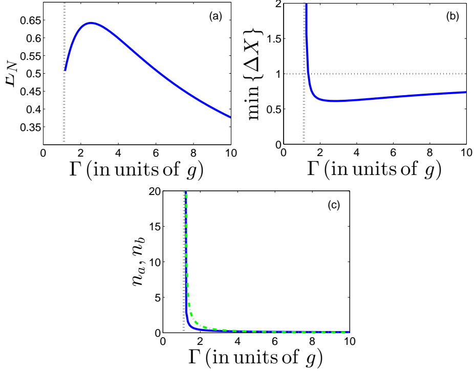
Figure 3.7: The same plots as in Fig. 3.6 with \kappa = 5g . In (c) the populations for the two modes are not equal and the two curves are not superimposed: the dark blue lines represent n_a and the light green lines represent n_b . Note that here, close the threshold value, the two-modes are entangled but the composite quadrature is not squeezed.
