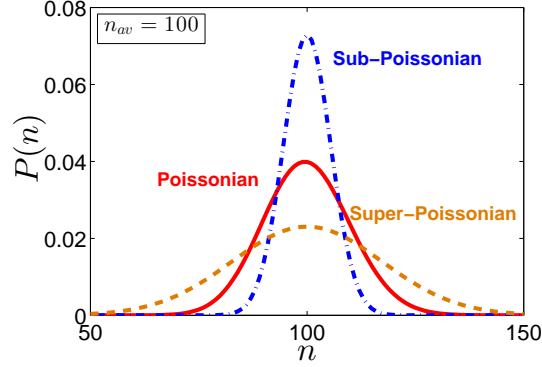
Figure 2.1: Plots of the probability P of finding n photons at a detector for a coherent light with Poissonian (red solid curve), anti-bunched light with sub-Poissonian (blue dotted-dashed curve), and bunched light with super-Poissonian (brown dashed curve) statistics. The average photon number n_{\text{av}} = 100 .
