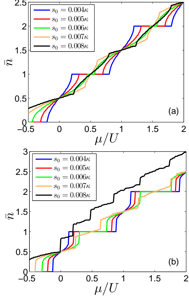
Figure 4.7: Mean density \bar{n} as a function of \mu (in units of \mu for a one-dimensional lattice of K = 100 sites for t = 0 , \delta_c = -5\kappa , u_0 = 0.8\kappa , U/\hbar = 50 Hz (with \kappa/2\pi = 1.3 MHz), while the values of s_0 are reported in the legend. The curves in (a) are evaluated by diagonalizing Eq. (4.41) after setting \langle \hat{\Phi} \rangle = 1/4 (i.e., by artificially removing cavity backaction). The curves in (b) are found for the corresponding parameters by diagonalizing the full quantum model of Eq. (4.41). The other parameters are as described in Fig. 4.5.
