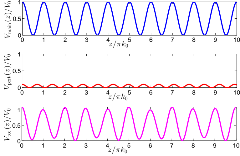
Figure 4.3: The quasi-periodic lattice potential V_{\text{tot}}(z) = V_{\text{main}}(z) + V_{\text{pert}}(z) which includes a main lattice potential V_{\text{main}}(z) = V_0 \cos^2(k_0 z) and a perturbative incommensurate lattice with V_{\text{pert}}(z) = \frac{V_0}{10} \cos^2(\sqrt{2}k_0 z) are plotted. The perturbative potential generates disorder to the main potential.
