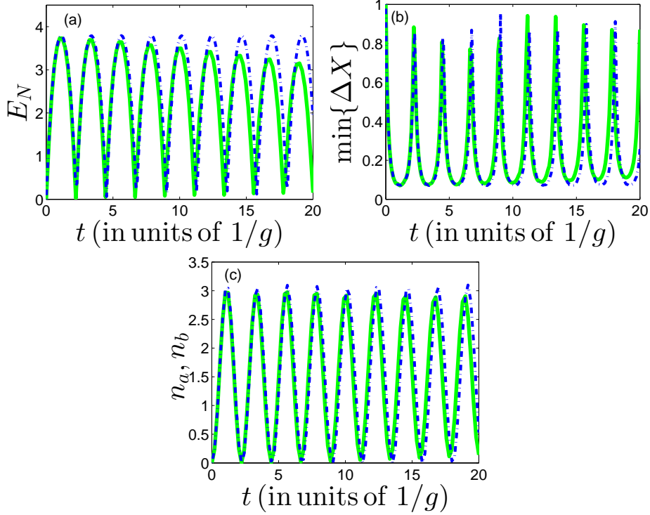
Figure 3.4: The same plots as in Fig. 3.3, but with \delta_c = -123.3g . The populations of the two-modes get larger with respect to Fig. 3.3 and hence for larger time, the effect of the four-wave mixing gets relevant in the dynamics.
