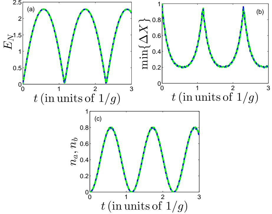
Figure 3.3: The same plots as in Fig. 3.1 with \omega_z = 100g, \Omega = 30g, N = 1000, \delta_c = -125g and the decay rates \kappa and \gamma are set to zero. The corresponding \delta_b = 118g . Here, due to a large value of N , the non-quadratic term in (3.7) due to four-wave mixing is negligible.
