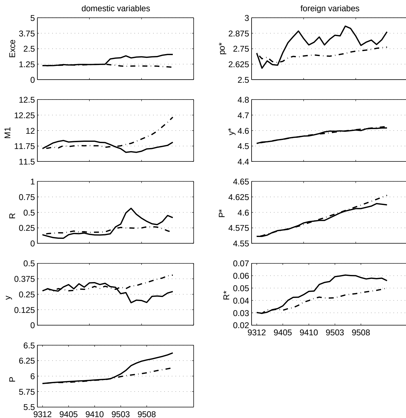
Figure 4: Actual and predicted value of domestic and foreign variables, 1993:12 - 1995:12
