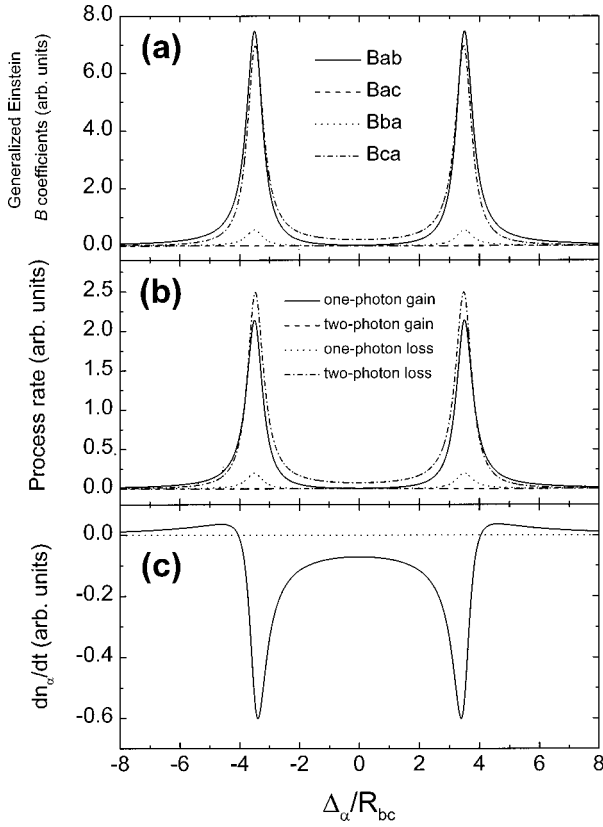
FIG. 6. As in Fig. 4 for the following set of parameters: R_{ab} = 0.1R_{bc} , R_{ba} = 0.08R_{bc} , \beta = 7R_{bc} , \Delta_\beta = 0 , and \alpha = 0.000\,02R_{bc} . The rest of the R_{ij} are taken as identically zero.
