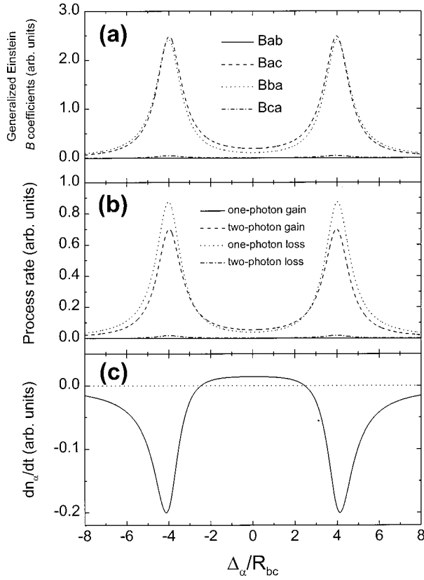
FIG. 8. As in Fig. 4 for the following set of parameters: R_{ac}=0.02R_{ab} , R_{ca}=0.8R_{ab} , \beta=8R_{ab} , \Delta\beta=0 , and \alpha=0.000\,02R_{ab} . The rest of the R_{ij} are taken as identically zero.
