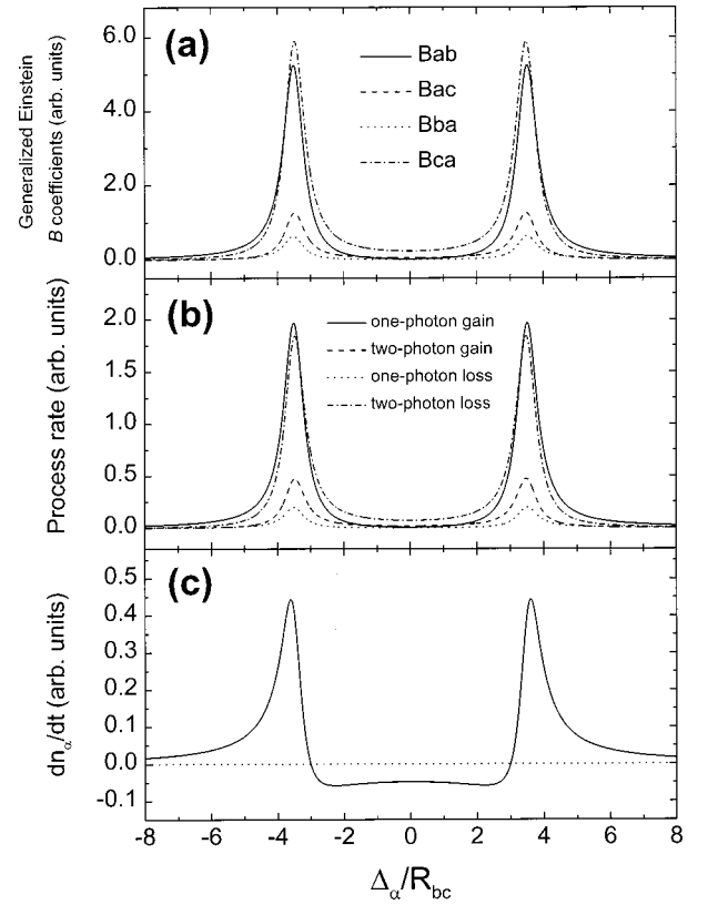
FIG. 7. As in Fig. 4 for the following set of parameters: R_{ac} = 0.1R_{bc} , R_{ca} = 0.12R_{bc} , R_{cb} = 0.12R_{bc} , \beta = 7R_{bc} , \Delta_\beta = 0 , and \alpha = 0.000\,02R_{bc} . The rest of the R_{ij} are taken as identically zero.
