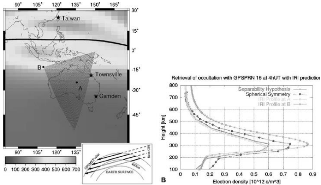
Figure 1. Typical GPSMET occultation near Australia. The ray parts between the GPSMET orbit and 400 km are marked separately from those under 400 km. The figure illustrates horizontal variation in electron density and compares spherical symmetry with the separability hypothesis.
