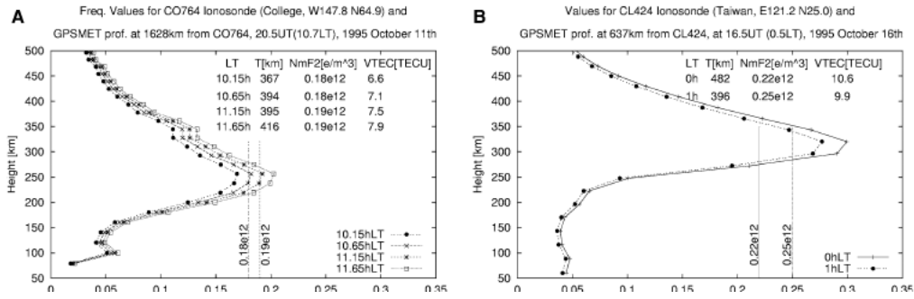
Figure 3. Effect of slab thickness in the comparison between ionosonde foF2 measurements and profiles retrieved from GPSMET data. Panel A shows an almost constant slab thickness; panel B shows a case where NmF2 increases while VTEC decreases.
