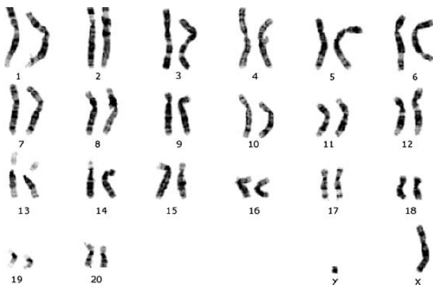
Figura 2. Cariotip del Mandril ( Mandrillus sphinx , 2n=42 )
