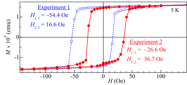
FIG. 1 (color online). Hysteresis loops at 5 K after applying and turning off 100 Oe magnetic field with “+” polarity (Experiment 1) and “-” polarity (Experiment 2) at 300 K and subsequent cooling down in the presence of remnant field of about -6 Oe. Note that the remnant field is superimposed on the applied field; hence the coercivity ( H_C ) values from the plots should be corrected correspondingly.
