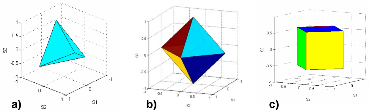
Figure 6. CN minimization for: (a) four, (b) six and (c) eight polarization analyzers. The vertexes of the regular polyhedrons are located upon the surface of the Poincare sphere.
