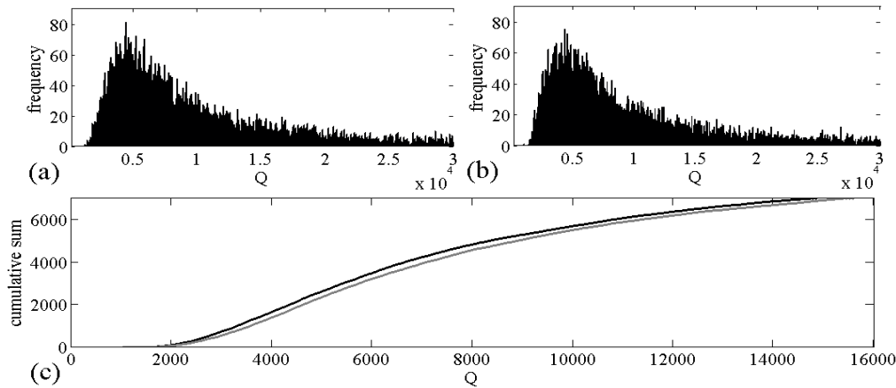
Figure 5. (a) and (b) Histograms of Q adding a random positioning error with standard deviation of 0.025 mm. not using and using NE, respectively. (c) Cumulative sum of the number of experiments with Q factor minor than the value of Q in x axis, using NE (black line) and not using NE (grey line).
