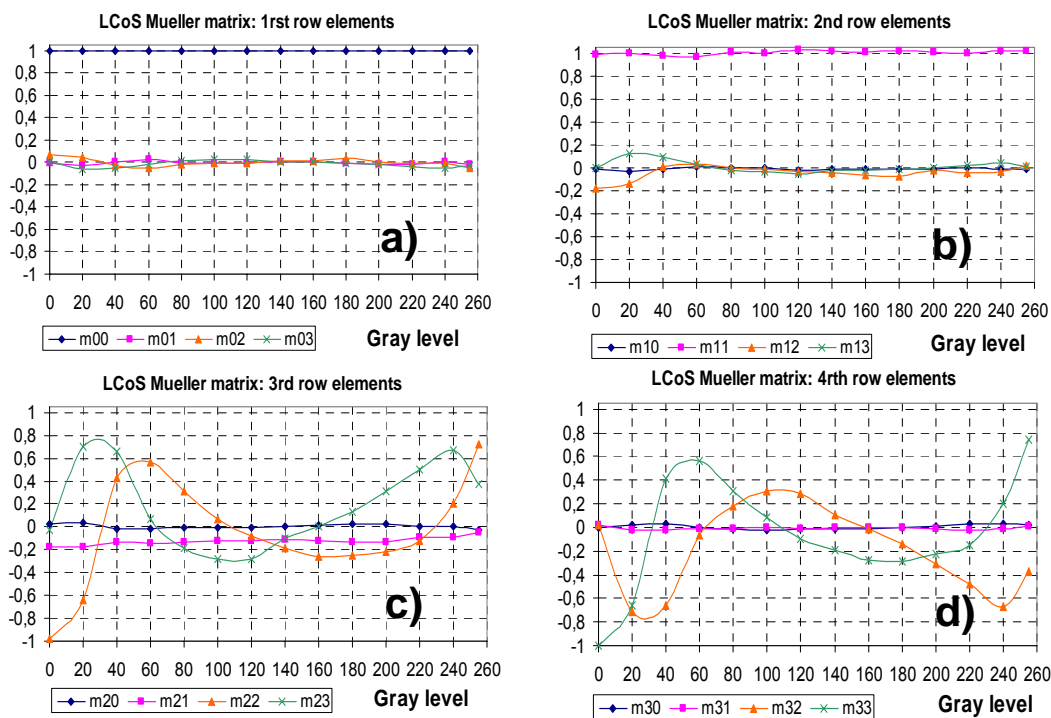
Figure 3. PA LCoS Mueller matrix experimental coefficients: a) First row elements; b) Second row elements; c) Third row elements; d) Fourth row elements.
