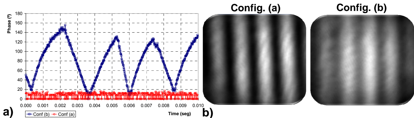
Figure 4. a) Time fluctuations of the phase for two configurations config.(a) and config.(b); b) Interference pattern detected when using two light beams with the gray levels 0 and 160 and the two different configurations.
