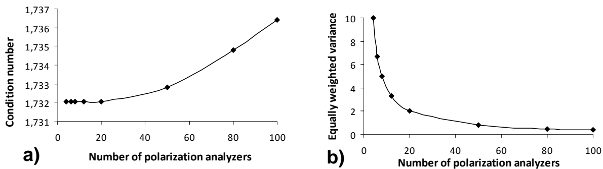
Fig. 7. Analysis of the CN (a) and EWV (b) as a function of the polarization analyzers number
