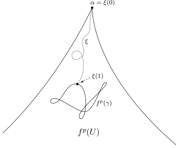
Figure 22: We can connect \alpha and f^p(\gamma) by a path \xi in f^p(U) \cup \{\alpha\} .
