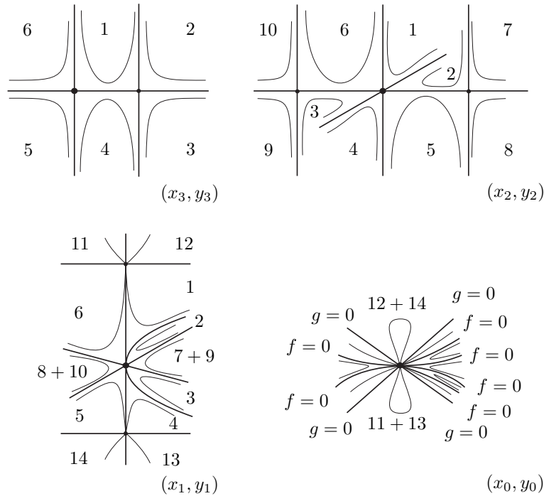
FIGURE 2. The desingularization of example 2.
