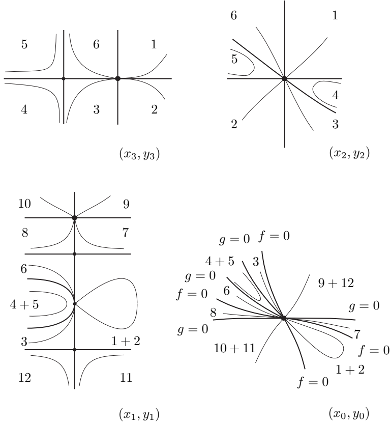
FIGURE 1. The desingularization of example 1. The numbers indicate the canonical regions of the systems to show how they change during the desingularization process. In each system the biggest point represents the origin.
