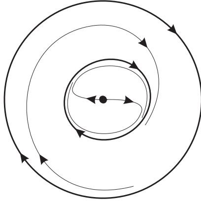
FIGURE 1. The phase portrait in the Poincaré disc of the polynomial differential system (2).
