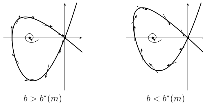
FIGURE 3. Negative and positive invariant regions around the focus
