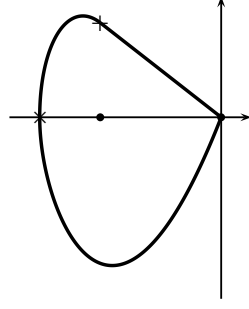
FIGURE 5. Piecewise loop for obtaining a negatively invariant region
