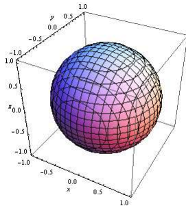
Elipsoide o esfera: x^2 + y^2 + z^2 - 1 = 0
