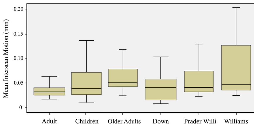
Fig. 1. Box-plots of head motion for the six study populations (after excluding group outliers). Group differences are apparent with regard to both the magnitude and range of motion. Mean and variance values for young adults (defined as the reference population) were significantly different from each of the other samples with p < 0.005 .
