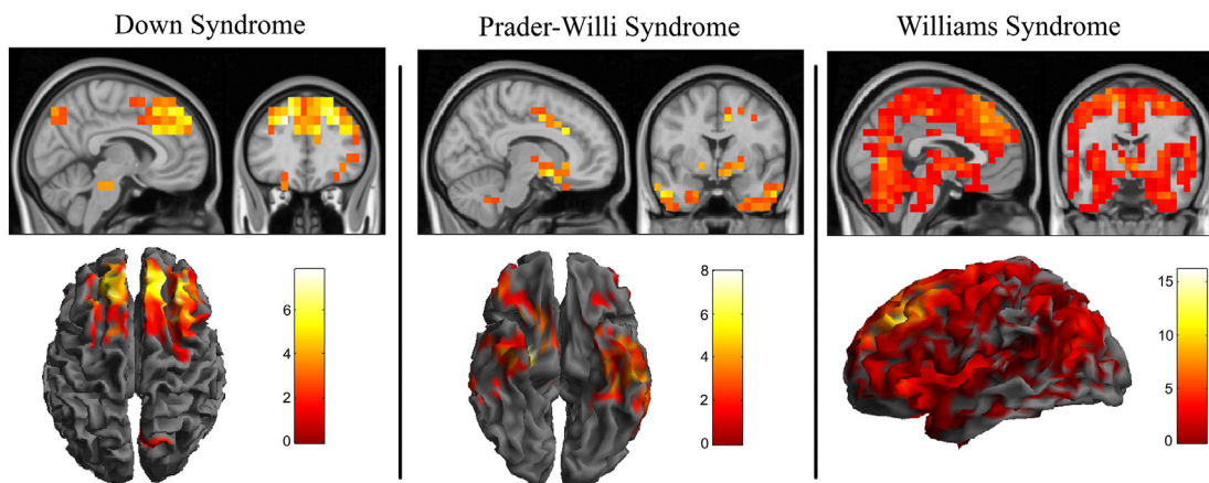
Fig. 6. Voxel-wise maps representing significant correlations between head motion and functional connectivity degree in patients with Down syndrome, Prader–Willi syndrome and Williams syndrome. Note the distinct distribution of correlations across these populations. Color bars correspond to t values.
