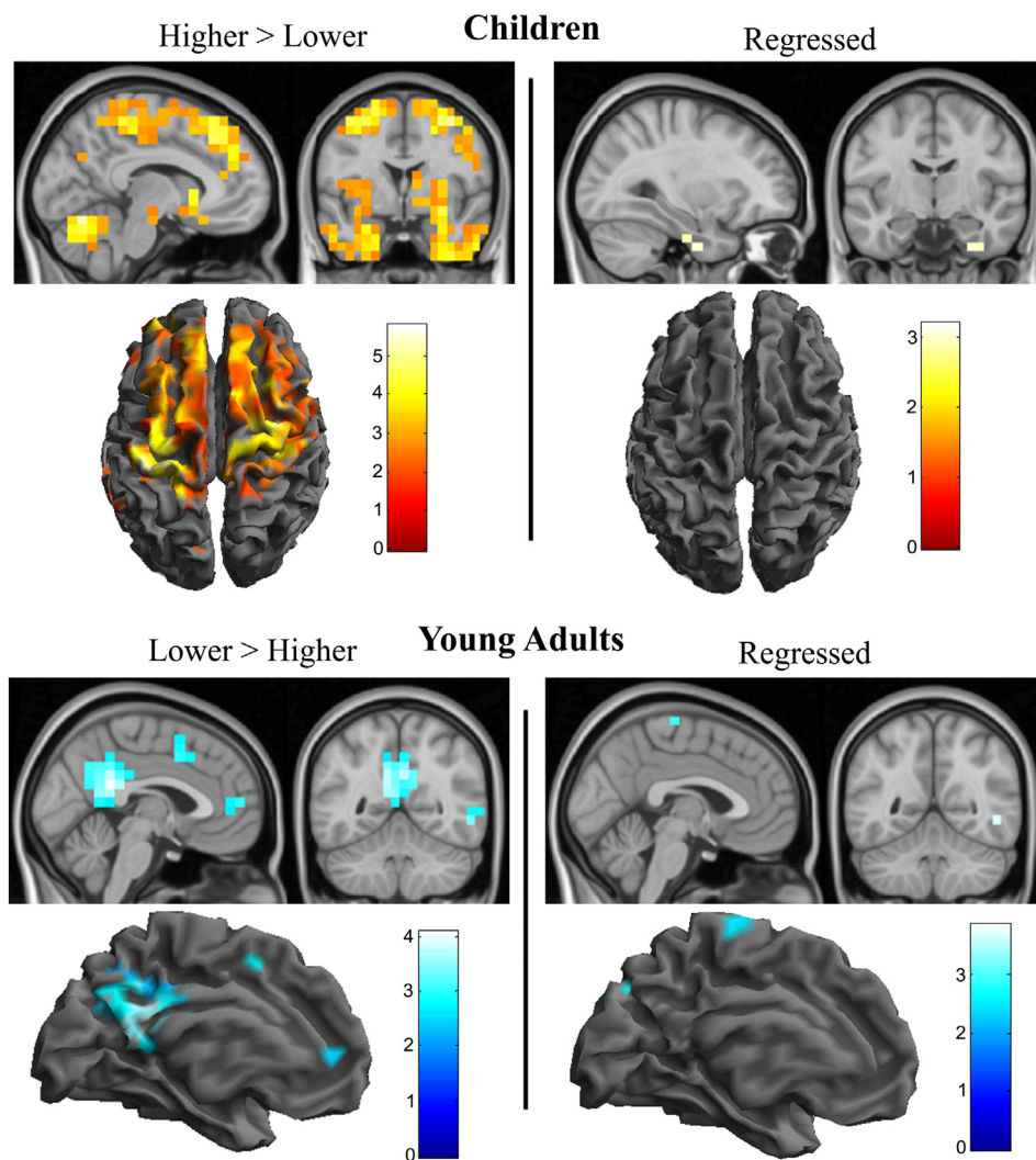
Fig. 7. Group-level removal of motion effects: Connectivity degree differences between the subgroup of children with higher ( n = 35 ) > lower ( n = 36 ) motion involved widespread brain areas. Including motion measurements as a covariate removed almost all of the observed subgroup differences. Similarly, connectivity degree differences between the subgroup of adults with lower ( n = 40 ) > higher ( n = 40 ) motion were mostly removed when applying this covariate. Color bars correspond to t values.
