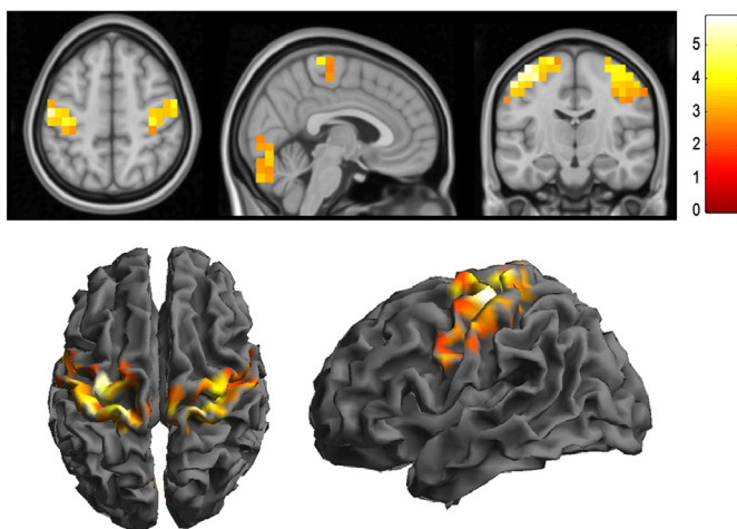
Fig. 3. Voxel-wise maps representing significant correlations between head rotation (combined x axis and z axis rotations) and functional connectivity degree in young adults. Note the precise involvement of the sensorimotor strip – extending from the feet to the neck and upper face cortical representation. Color bars correspond to t values.
