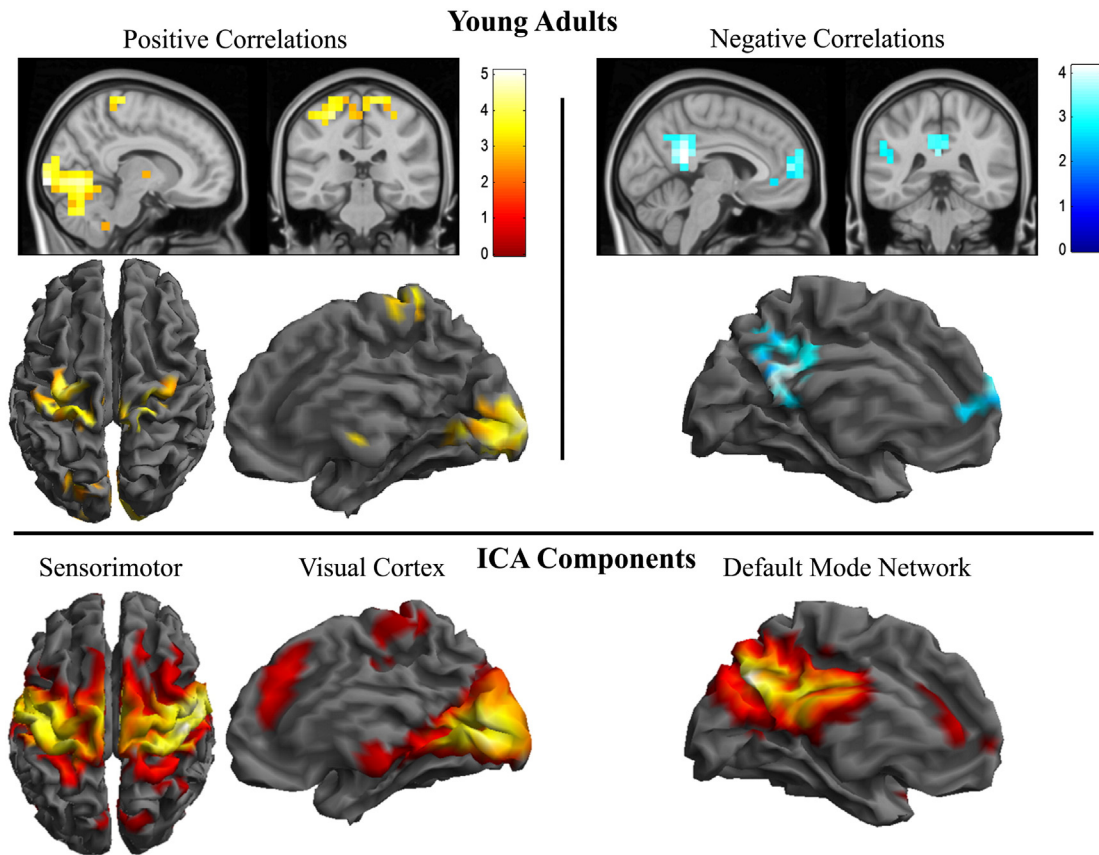
Fig. 2. Voxel-wise maps representing significant correlations between head motion and functional connectivity degree in young adults. Positive correlations involved the sensorimotor and visual cortices bilaterally. Negative correlations involved core areas of the default mode network including the posterior cingulate and medial frontal cortices. Color bars correspond to t values. An independent component analysis (ICA) was used to identify the implicated resting-state functional networks (bottom panel). Note the clear overlap between motion/connectivity correlation results and core regions of the ICA-estimated functional networks.
