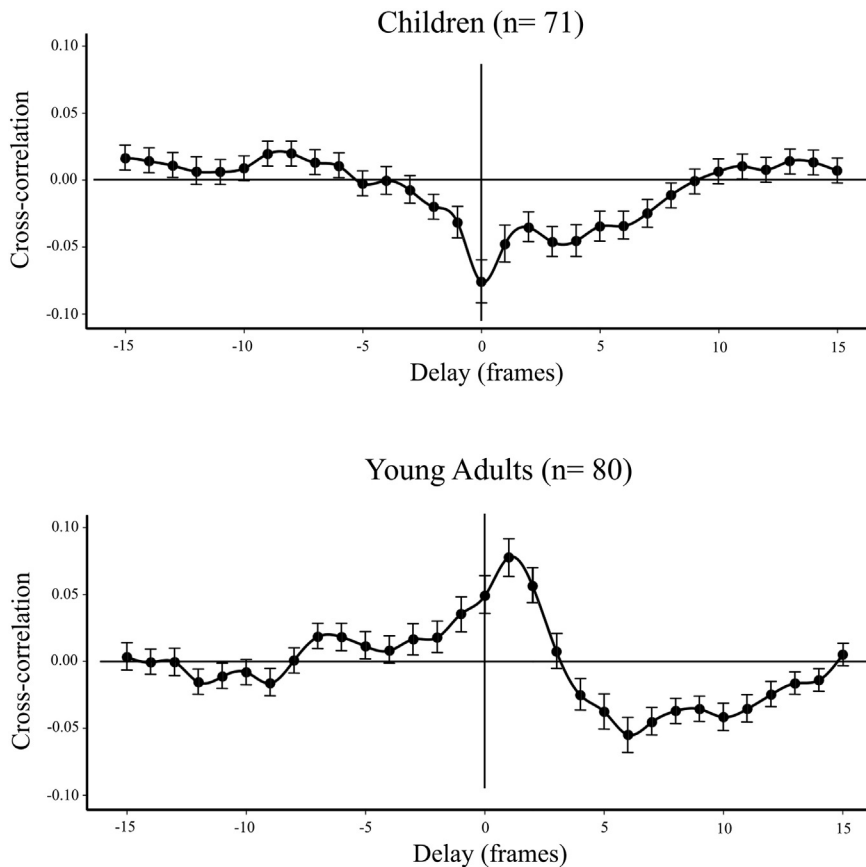
Fig. 4. Group results from the cross-correlation analysis. The temporal evolution of inter-frame head motion was correlated with the fMRI signal time course (group mean cross-correlation r values with \pm standard error of mean in axis y ). The correlation was repeated after applying 1 frame (2 s) time-lags to the motion time course both forward (positive values in axis x ) and backward (negative x values). In children’s dorsal frontal cortex (MNI -12, 38, 44 ), the largest negative correlation at zero delay (i.e., signal decrease temporally coinciding with motion) suggests an artifactual effect. In young adults, by contrast, motion was positively correlated with fMRI signal of the motor cortex (MNI -25, -18, 68 ) at zero time-lag and also when applying motion time course delays up to 2 frames (4 s). This pattern suggests a coupling of motion with hemodynamically delayed fMRI signal increase related to neural activity.
