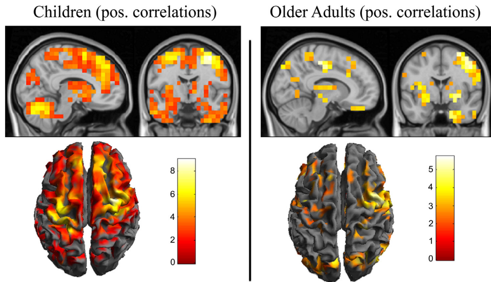
Fig. 5. Voxel-wise maps representing significant correlations between head motion and functional connectivity degree in children and older adults. Significant correlations involved widespread areas in both groups, although children showed the most pronounced effects. Color bars correspond to t values.
