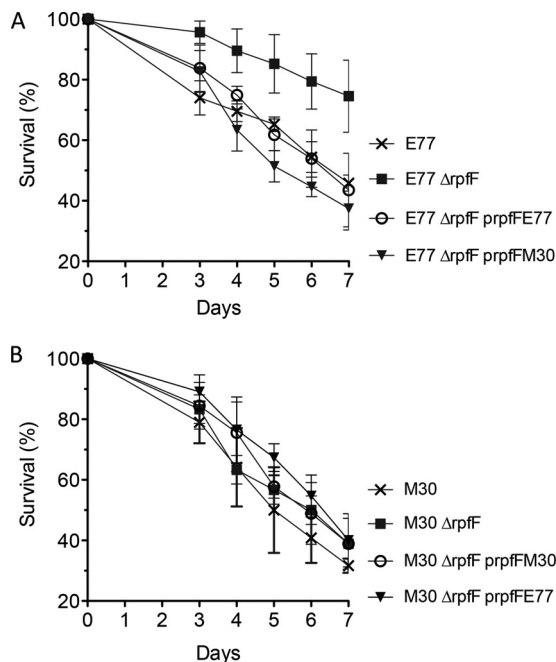
FIG 8 Determination of virulence of E77 (A), M30 (B), and their respective \Delta rp f F mutants and homologously and heterologously complemented strains in a C. elegans CF512 model of infection.
