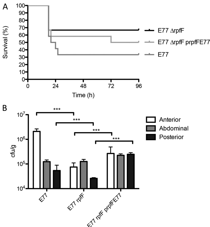
FIG 9 (A) Virulence of E77, the \Delta rp f F mutant, and the complemented strain in 9-month-old zebrafish. (B) Bacterial recovery from different regions of the bodies of sacrificed fish at 72 h postinfection with E77, the \Delta rp f F mutant, or the complemented strain. ***, P < 0.0005 .
