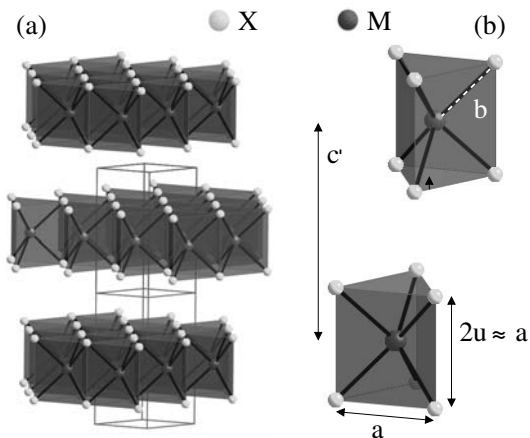
FIG. 1: (a) Schematic representation of the atomic structure of MX_2 . The bulk compound has a 2H- MX_2 structure with two MX_2 layers per unit cell, each layer being built up from a trigonal prism coordination unit. The small green rectangle represents the unit cell of a monolayer of MX_2 , which is doubled (red extension) in the bulk crystal. (b) Detail of the trigonal prisms for the two layers in the bulk compound, showing the lattice constants and the definition of the structural angles used in the text.
