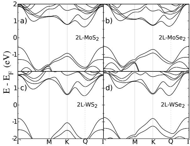
FIG. 4: Band structure of bilayer \text{MoS}_2 , \text{MoSe}_2 , \text{WS}_2 and \text{WSe}_2 obtained from DFT calculations.
