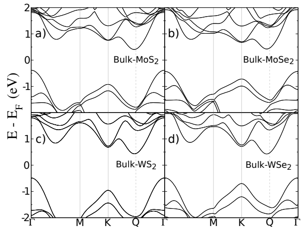
FIG. 3: Band structure of bulk MoS 2 , MoSe 2 , WS 2 and WSe 2 obtained from DFT calculations.
