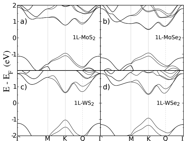
FIG. 2: Band structure of single layer MoS 2 , MoSe 2 , WS 2 and WSe 2 obtained from DFT calculations, including SOC. Dashed vertical lines indicate the position of the Q point in the BZ (see text).
