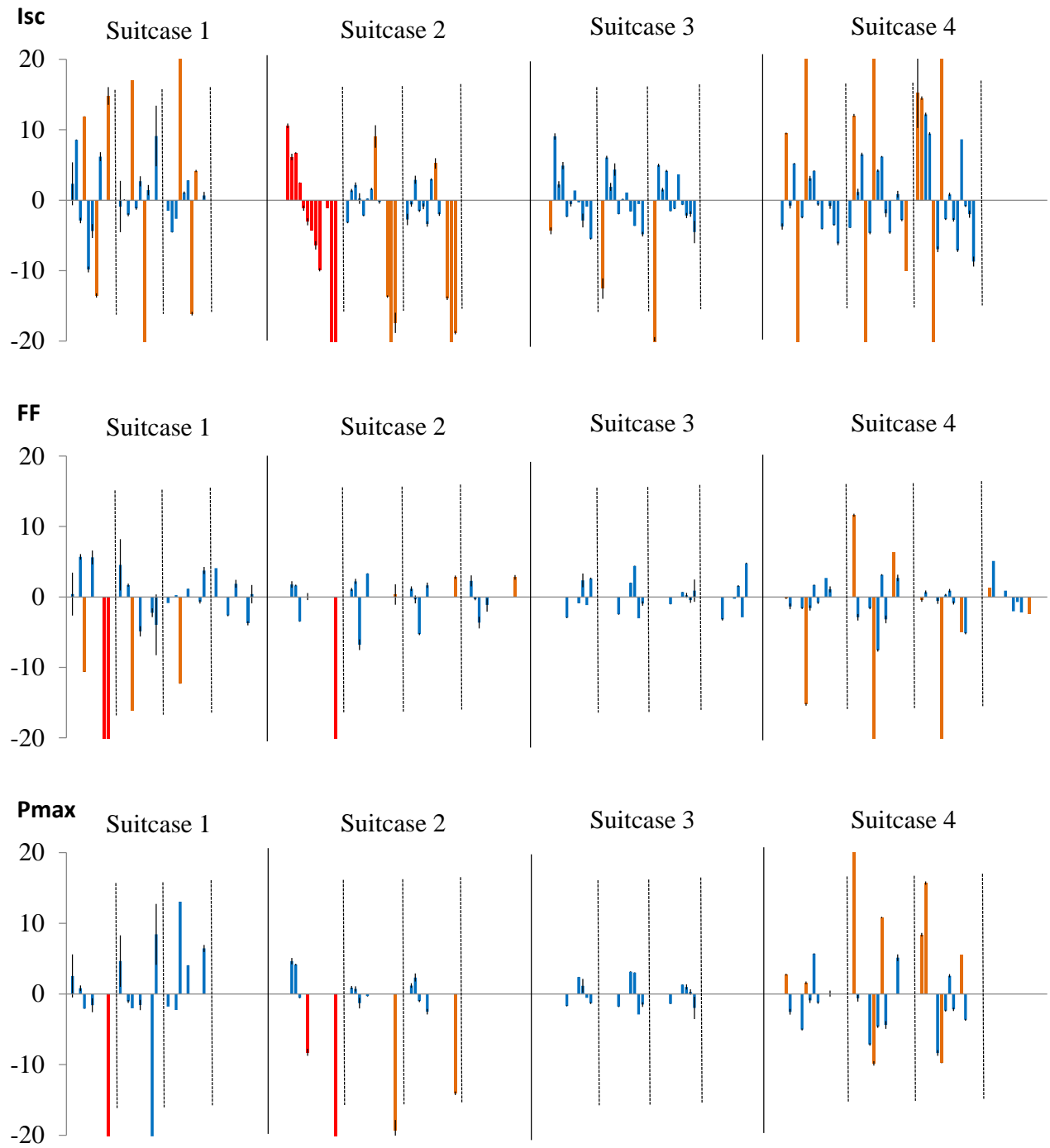
Figure 6. Deviations of reported PV parameters for all the laboratories for each suitcase. The orange columns represent the data that was qualified as an outlier due to extreme testing conditions. The red columns represent the data of degraded devices.
