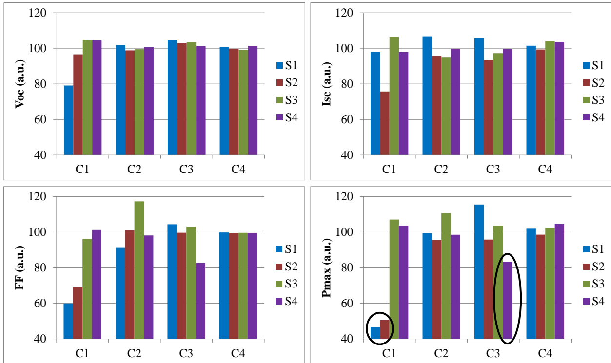
Figure 5. Performance of all the samples after the experiments normalized to the initial values. C1 to C4 refer correspondingly to Cell 1 to Cell 4 in each suitcase (Table 1). The three samples which showed degradation are marked with a black circle.
