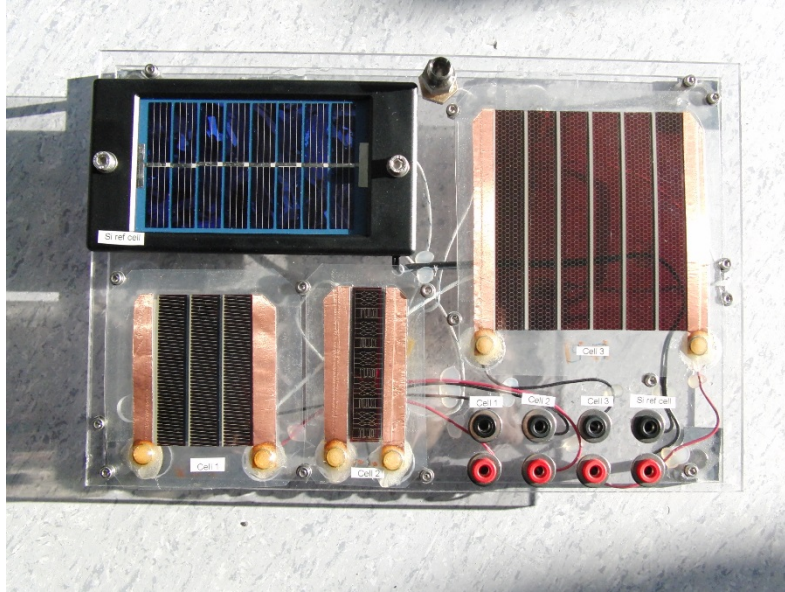
Figure 1: Three OPV modules and one Si reference module fixed on a rigid platform
