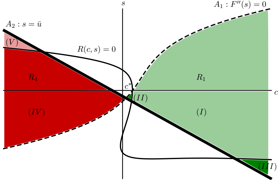
Figure 6: Choosing parameters in the lighter shaded regions (I) and (V) we obtain solitary waves which increase with the wave speed c , whereas solutions corresponding to parameters in the darker shaded regions (II), (III) and (IV) decrease with respect to c .
