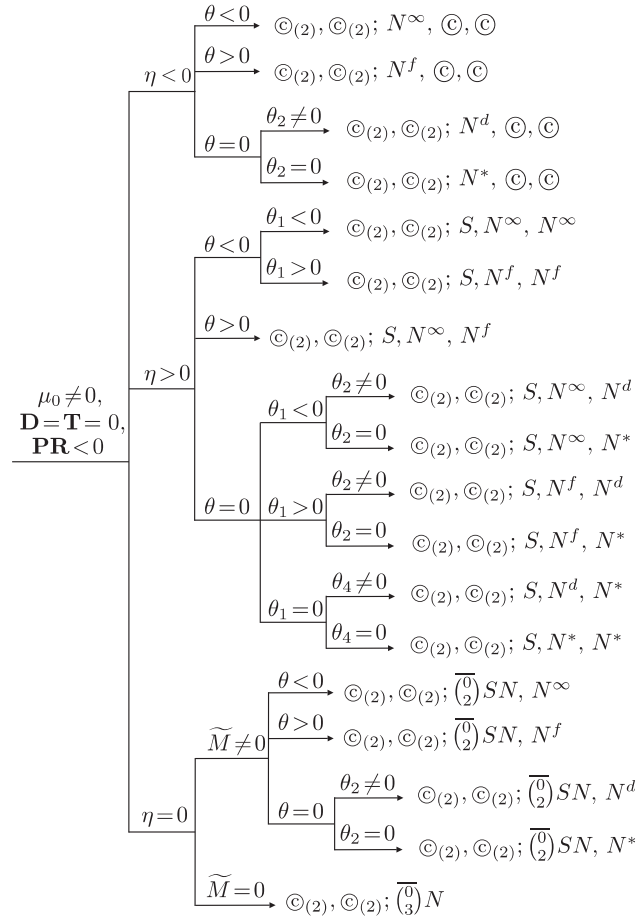
DIAGRAM 1. Global configurations: the case \mu_0 \neq 0, \mathbf{D} = \mathbf{T} = 0, \mathbf{PR} < 0 .
