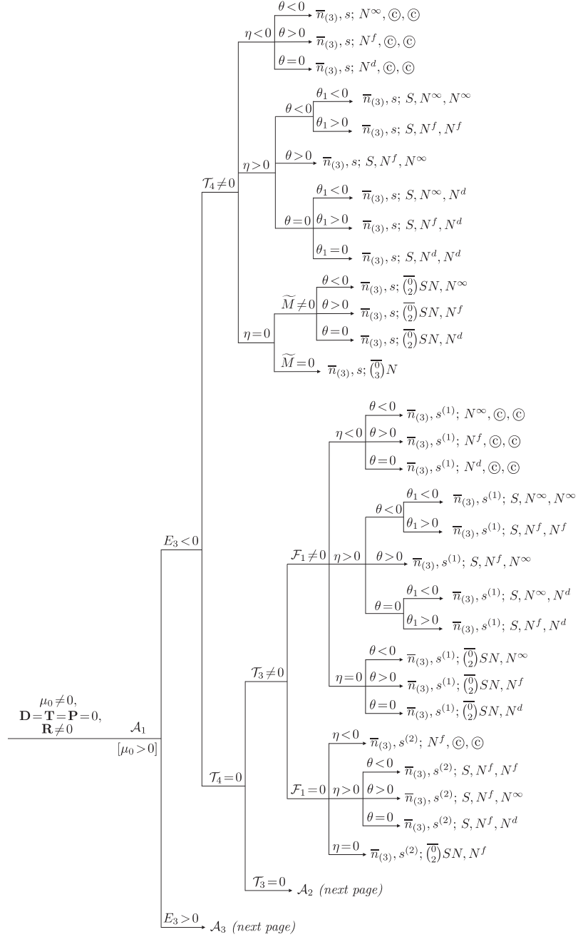
DIAGRAM 3 (continued). Global configurations: the case \mu_0 \neq 0 , D = T = P = 0 , R \neq 0 .
