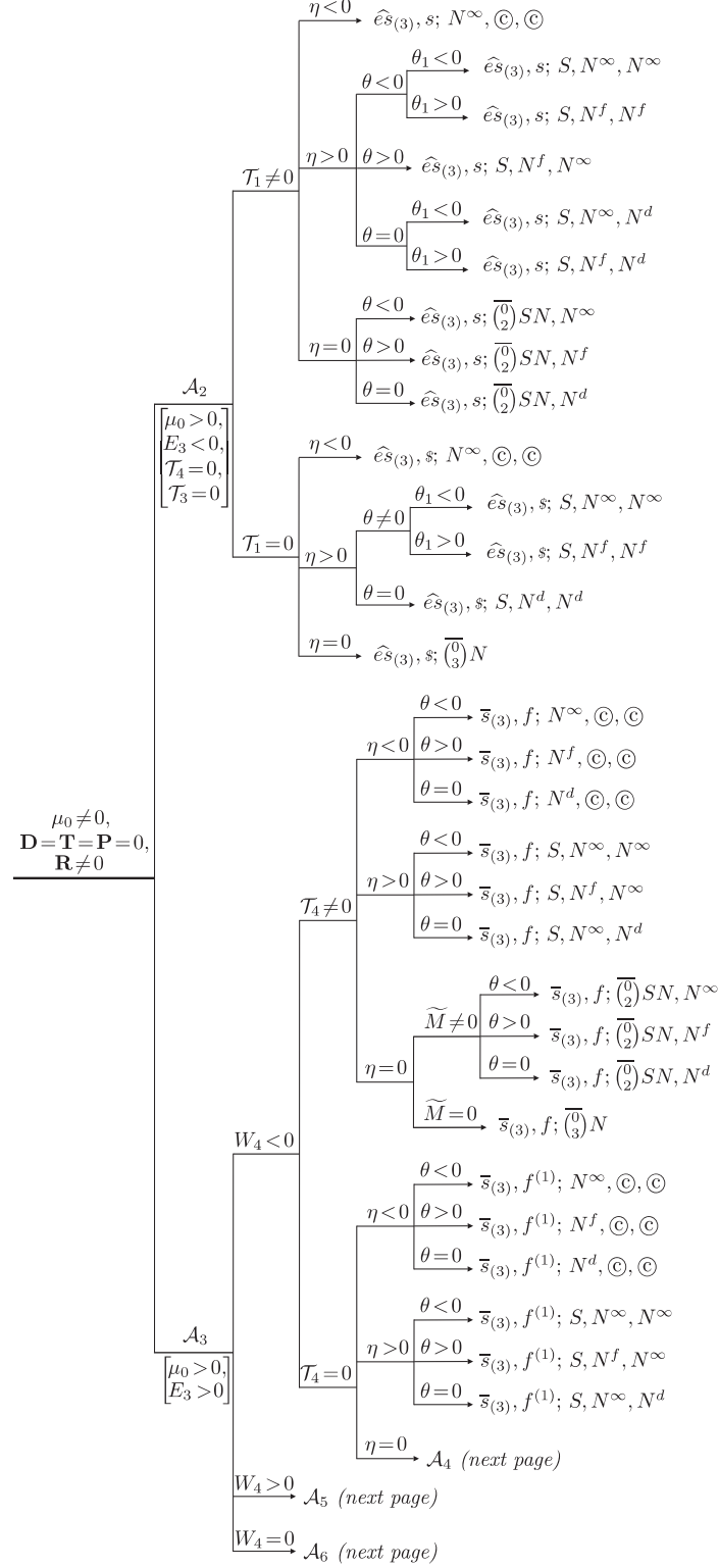
DIAGRAM 3 (continued). Global configurations: the case \mu_0 \neq 0 , D = T = P = 0 , R \neq 0 .
