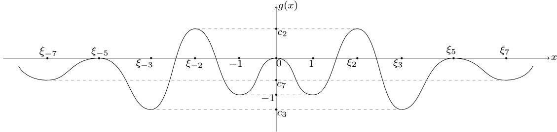
FIGURE 4. Sketch of a Laguerre-Pólya function g on the real line, with the choices c_0 = 0 , c_{\pm 1} = -1 , c_{\pm 4} = c_{\pm 5} = c_{\pm 6} = 0 and c_n = c_{-n} for all n \in \mathbb{N} . Consequently we may normalize so that \xi_{\pm 1} = \pm 1 and \xi_0 = 0 . We also have multiple critical points \xi_4 = \xi_5 = \xi_6 and \xi_{-4} = \xi_{-5} = \xi_{-6} .
