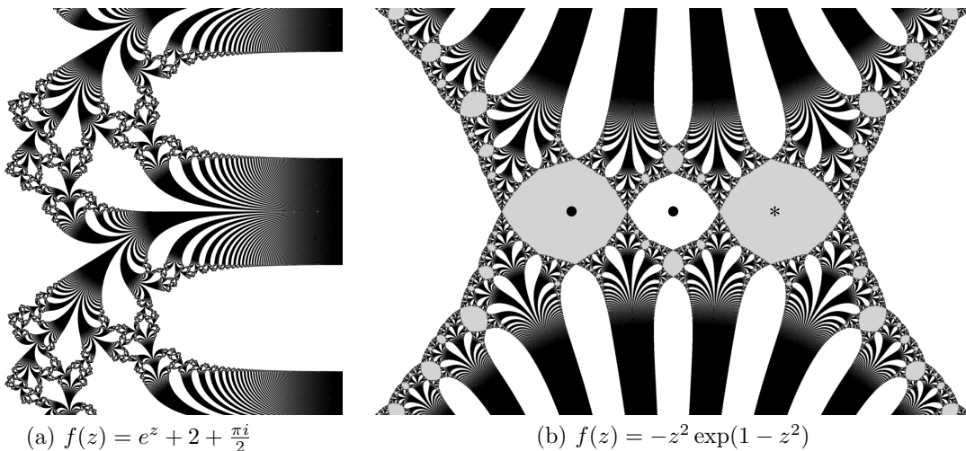
FIGURE 1. Two entire functions with asymptotic values and unbounded Fatou components (the Julia set is drawn in black; Fatou components are in white). On the left is an exponential map; the Fatou set consists of the basin of an attracting orbit of period 3. Every Fatou component U is unbounded and \partial U is not locally connected. On the right is a function that plays a crucial role in our construction of Example 1.6. Here there are superattracting fixed points at 0 and -1 (marked with filled circles), and 0 is an asymptotic value. The basin of 0 is coloured white and the basin of -1 is coloured grey – every Fatou component is a Jordan domain, but all pre-periodic components of the basin of 0 are unbounded, and the Julia set is not locally connected. Here and in subsequent images, non-periodic critical points (in this case, the point 1) are marked by asterisks.
