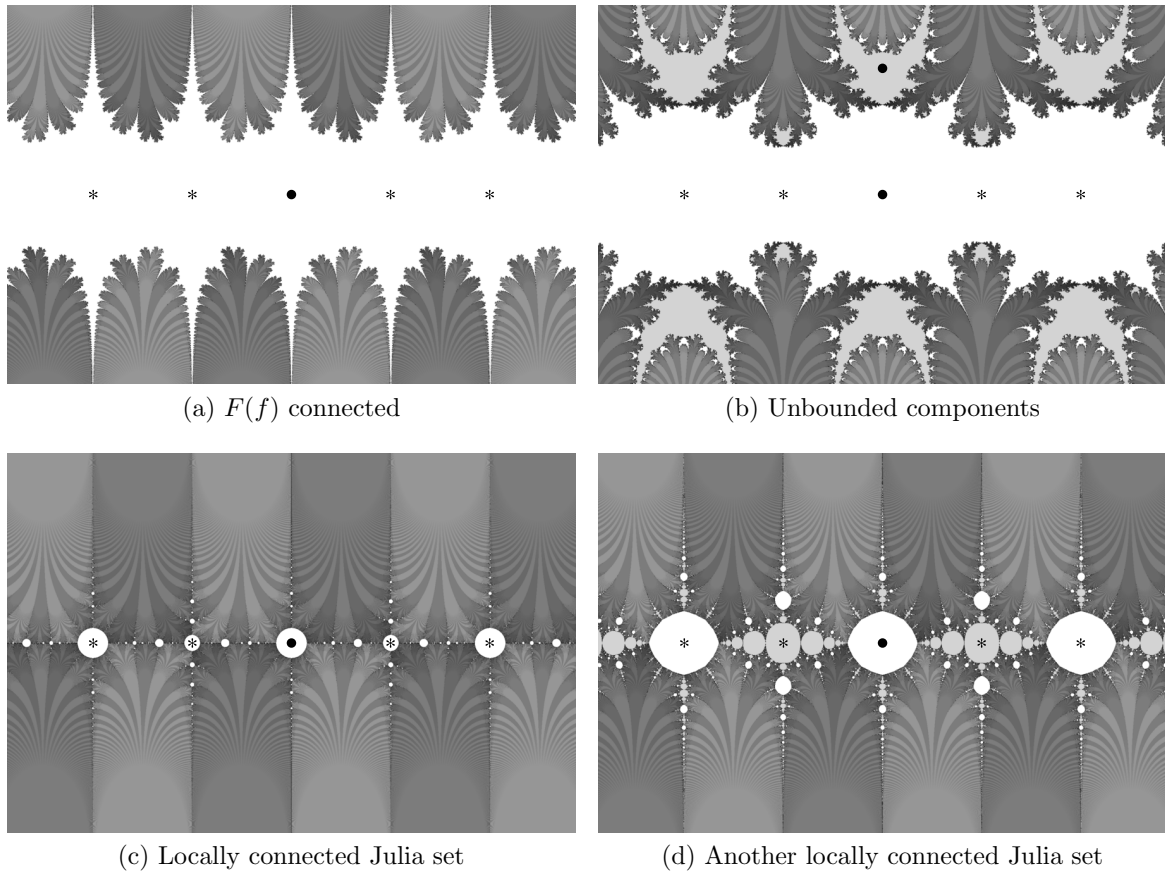
FIGURE 2. Julia sets (in dark grey) of some maps in the cosine family, z \mapsto a \cos(z) + b , illustrating Theorem 1.4 and Corollary 1.9. 1 (Note that these can easily be reparametrised as z \mapsto \sin(a'z + b') for suitable choices of a', b' .) The two maps in the top row have unbounded Fatou components and their Julia sets are not locally connected. The maps on the bottom line both have locally connected Julia sets.
