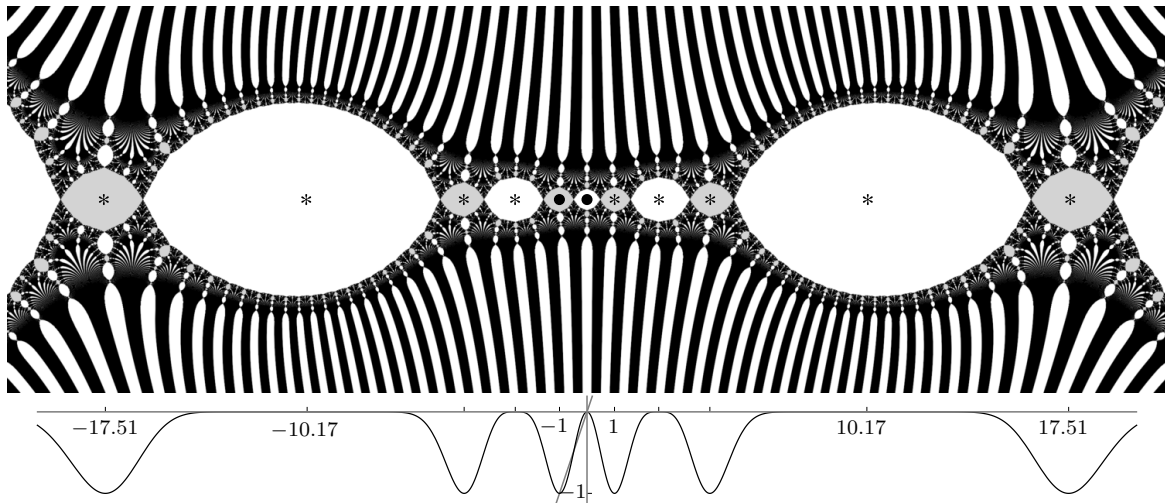
FIGURE 5. Illustration of the construction of Example 1.7. Shown are the Julia set and the graph of the function g_2 that would arise from the choice of N_1 = 5 and N_2 = 25 . Note the large size of the Fatou components containing high-degree critical points. For the actual construction of Example 1.7 the sequence (N_k) has to grow much more rapidly than indicated by the above values of N_1 and N_2 .
