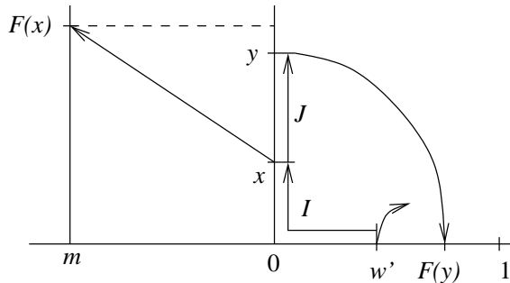
FIGURE 9. Intervals I and J , with arrows indicating their order. Though not needed in the proof, it can be noticed that the assumptions imply that r(F(w)) \in (0, 1) , and hence F(y) = F(w) \in (0, 1) .
