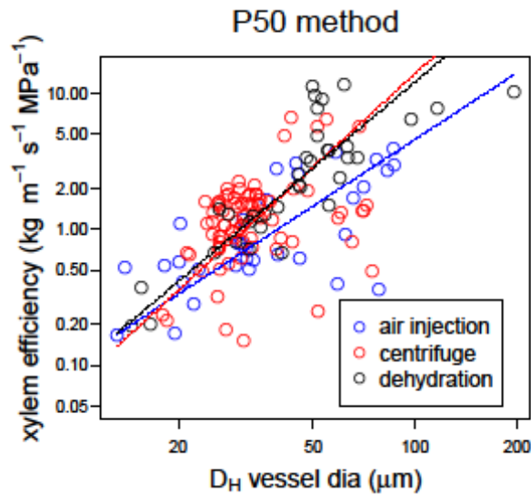
Fig. S7 Comparison of methods used for generating P_{50} data. Trendlines exhibiting significantly higher elevation indicates greater efficiency at a given hydraulically weighted vessel diameter and therefore suggests a methodological artifact. Only methods which reported both efficiency and hydraulically weighted vessel diameter are included here. ‘Air injection’ includes the double-ended method only. ‘Centrifuge’ does not include data collected using the Cavitron method (Cochard, 2002).
