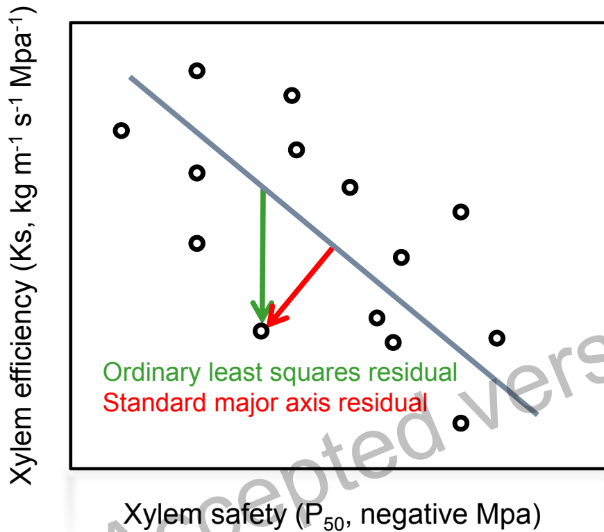
Fig. S1 Standard major axis residuals (SMA) vs. ordinary least squares (OLS) residuals. Note that SMA residuals include variation on both the x and y axes, whereas OLS residuals include only variation on the y axis. As such, OLS residuals reflect variation orthogonal to x, whereas SMA residuals reflect variation orthogonal to the y \sim x fit. By plotting the third variable against the efficiency~safety SMA residuals, the degree to which the third variable modifies the efficiency~safety relationship can be assessed.
