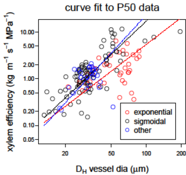
Fig. S6 Comparison of ‘curve shapes’ exhibited by fitted bivariate models (i.e., P_{50} curve) for angiosperm species in the database. Trendlines with significantly higher elevation coefficients indicate greater efficiency at a given hydraulically weighted vessel diameter, and therefore, suggests a methodological artifact. However, although exponential curves are thought to be associated with “open” vessels (i.e., less resistance), samples fit with exponential curves tended to have lower efficiency, not higher.
