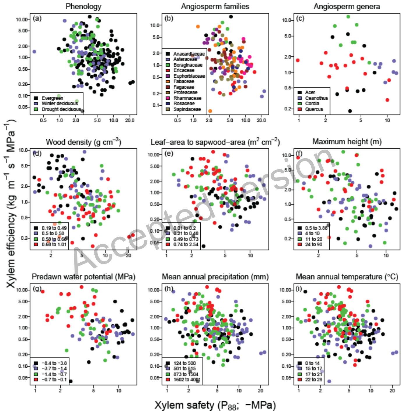
Fig. S2 Hydraulic efficiency-safety ( P_{88} ) plots for angiosperm species. Axes have been log10 scaled. Different colours represent different leaf habits (panel a), taxonomic groups (panels b, c), plant structural traits (panels d, e, f), and site factors (g, h, i). Continuous variables were binned in roughly equal groups of four with bin ranges denoted in the legends.
