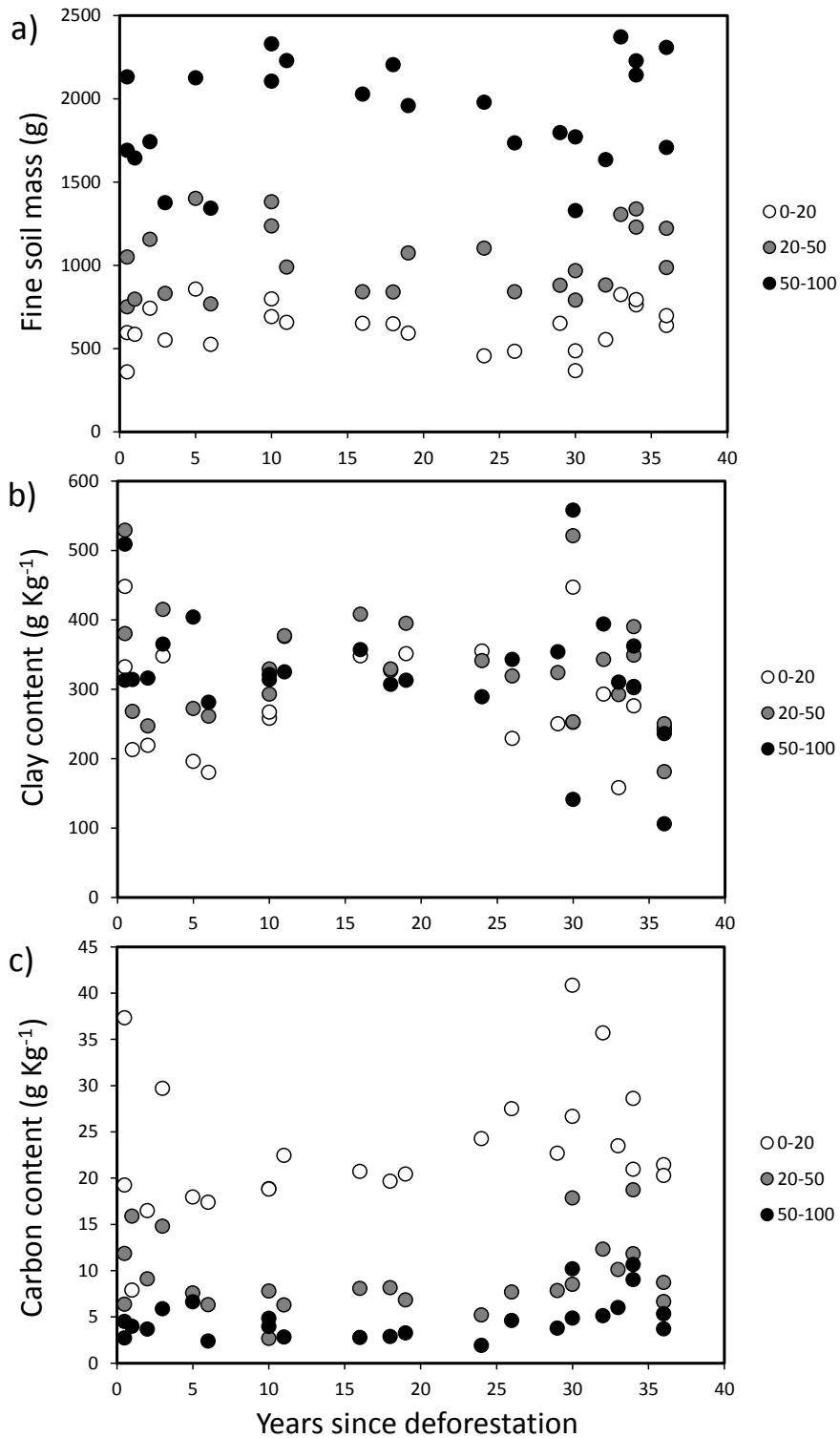
Figures1: Soil characteristics for each pasture along the chronosequence : a) fine soil mass (g), b) clay content (g kg -1 ) and c) carbon content (g kg -1 ) in each soil layers. Open circle is the 0-20 cm soil layers, grey circle is the 20-50 cm soil layer and the closed circle is the 50-100 cm soil layer.
