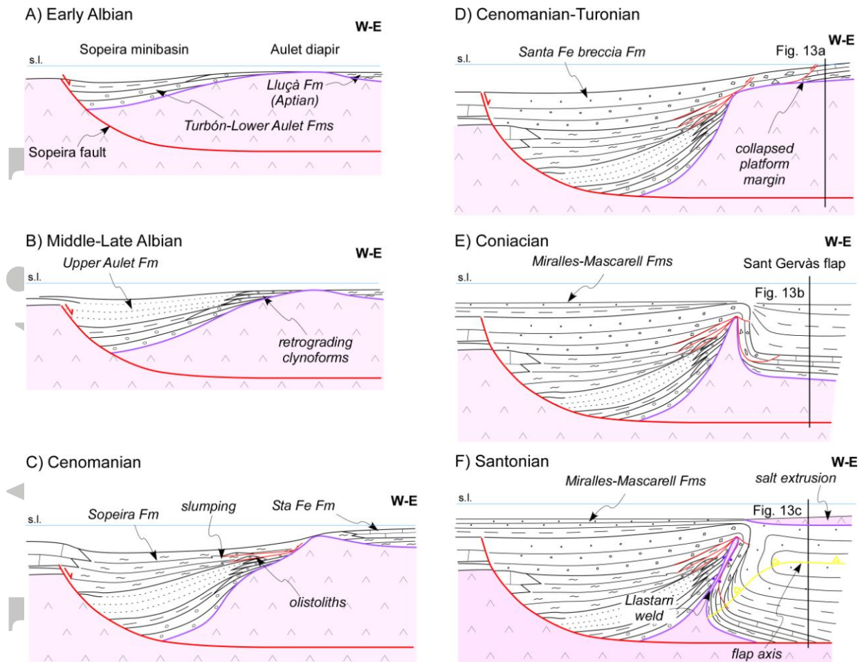
Fig. 12. Synthetic evolutionary model showing the shift of the main depocenter from Sopeira to Sant Gervàs depocenters at the Cenomanian-Turonian transition. From Turonian to Santonian the fall of the Aulet diapir leads to the welding of its roof and wall forming the Llastarri weld (see text for explanation).
