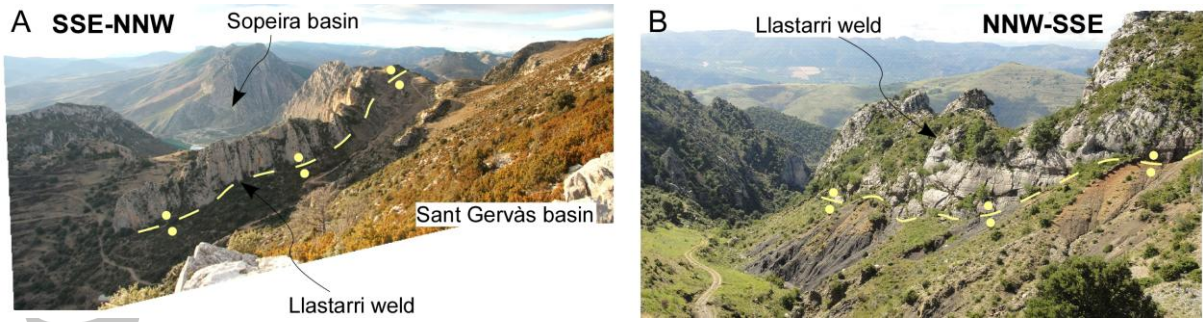
Fig. 7. A) The N-S Llastarri weld from the east. The limestone ridge corresponds to the base of the retrograding Aulet Formation clinoforms of the Sopeira basin lapping onto the former Aulet diapir. B) Detail of the N-S Llastarri weld showing large-scale groove marks (subhorizontal) evidencing tectonic displacement between the weld walls. See Fig. 6a for location.
