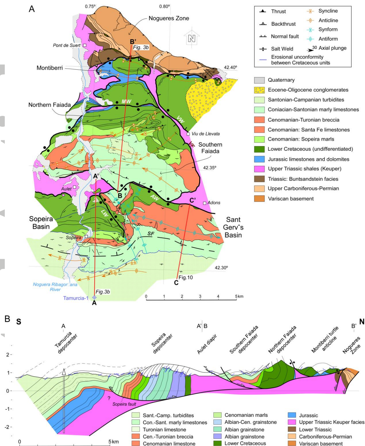
Fig. 3. A) Geological map of the Ribagorça basin. AW – Aulet weld; LW – Llastarri weld; MW – Montiberri weld; VW – Viu weld; SF – Sopeira Fault, VF – Viu Fault. B) Cross-section across the Sopeira, Tamurcia, Faiada and Montiberri basins. Note that the section extends outside the map area, 2.6 km south of the Tamurcia-1 well.
