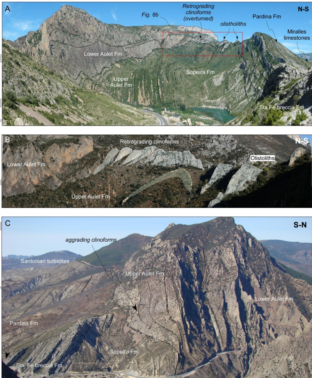
Fig. 8. A) Eastern side of the Sopeira basin. The Upper Aulet grainstone in the foreground, grades to a system of retrograding clinoforms in the background. The Sopeira marls thin eastwards where they interbed with a system of olistoliths made of Lower Aulet grainstone limestone. While in the foreground the succession is in upright position with decreasing dip southwards, in the background the succession is mostly overturned. B) System of retrograding clinoforms and possibly gravitational olistoliths defining the eastern margin of the Sopeira basin, attached to the N-S Llastarri weld. The view shows the subvertical to overturned top of the clinoforms, which deepen towards the left of the picture. C) Western side of the Sopeira basin where the Albian-Cenomanian succession displays an upright attitude and an upsequence decrease of bedding dip. The Aulet Formation beds define a system of east-facing aggrading clinoforms on top of which lap the beds of the Sopeira Formation that thins westwards. The upper part of the succession is truncated by the Santonian Mascarell turbidites, marking the early compressional folding of this segment of the Pyrenees. See Fig. 6a for location.
