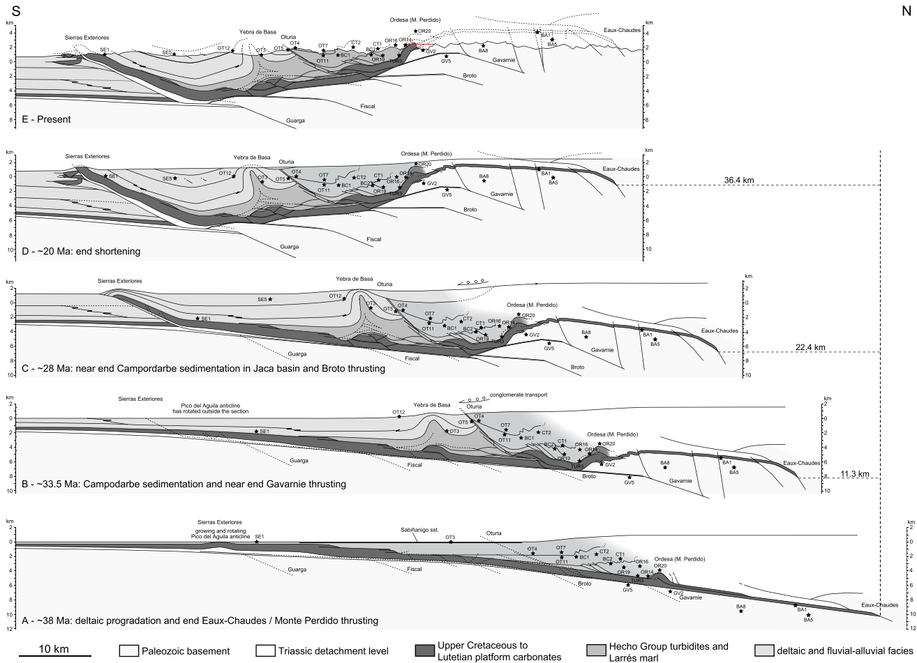
Figure 14. Model for the tectonic evolution of the eastern Jaca Basin and southern Axial Zone, corresponding to the sequential restoration of the cross section in Figure 5. See detailed legend in Figure 5.
