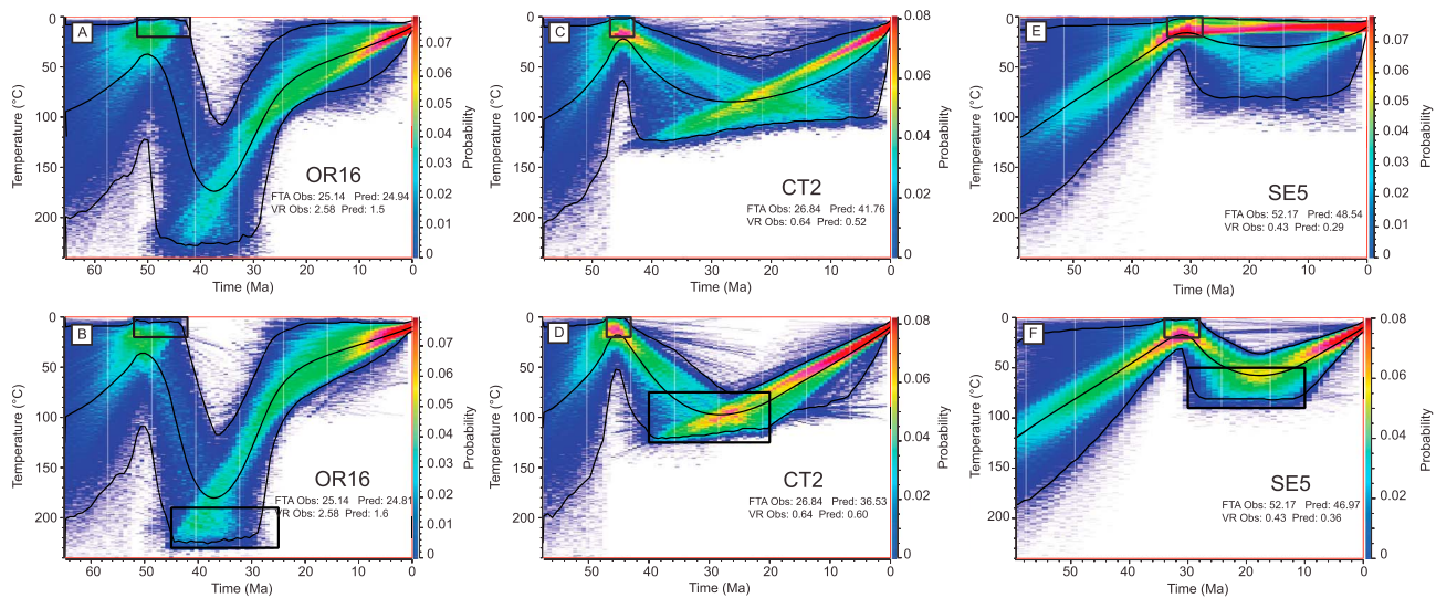
Figure 13. Statistic inverse modeling of the AFT and vitrinite reflectance data for three selected samples from the Jaca Basin. Models were obtained using the QTQt software [Gallagher, 2012]. The temperature-time constraints are indicated by black rectangles and correspond to the estimated stratigraphic age of the sample in a (a, c, and e) first set of models, complemented by the vitrinite-derived temperature at the estimated time of maximum burial (with an error margin of \pm 10 Ma) in (b, d, and f) a second set. The black line represents the mean expected model cooling curve [Gallagher, 2012], and the blue to red color scale describes the probability of the cooling curve to pass through a given temperature-time point. FTA Obs is the observed AFT central age, and FTA Pred is its predicted value; VR Obs is the observed vitrinite reflectance value, and VR Pred is the value predicted by the model. See text for discussion.
