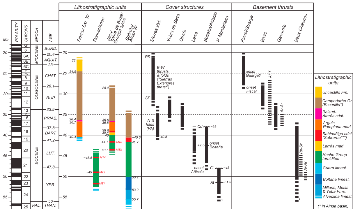
Figure 4. Table presenting a synthesis of the ages of stratigraphic units and timing of activity of the major tectonic structures of the Jaca Basin and adjacent Axial Zone. Stratigraphic ages are compiled from previous magnetostratigraphic and biostratigraphic studies with absolute ages of chrons and stratigraphic divisions corrected according to recent timescales [Gradstein et al., 2012; Cohen et al., 2013]. Timing of cover structures (deduced from growth strata and angular unconformities) are compiled from previous studies and additional own field observations. Timing of basement thrusts are based of geometrical features and displacement transfer considerations as discussed in the text. References for stratigraphic units: Hogan and Burbank [1996]; Labaume et al. [1985]; Mochales et al. [2012]; Oliva-Urcia et al. [2015]; Oms et al. [2003]. References for cover structures: Hogan and Burbank [1996], Labaume et al. [1985], Poblet and Hardy [1995], Teixell [1996], Muñoz et al. [2013], and Oliva-Urcia et al. [2015]. AFT: apatite fission track ages in the Néouvielle [Jolivet et al., 2007] and Balaitous (this work) granites; Ar-Ar: 40 Ar/ 39 Ar ages of K-feldspar in shear zones in the Néouvielle granite [Jolivet et al., 2007] and authigenic illite from shear zones in the Gavarnie thrust fault zone [Rahl et al., 2011]; At: Atiart unconformity; Cd: Campodarbe unconformity; CL: Charro-Lascorz unconformity; PA: Pico del Aguila anticline; PS: Peña del Sol thrust; Rb/Sr: Rb-Sr ages of shear zones in the Néouvielle granite [Wayne and McCaig, 1998]; and SF: San Felices thrust. The Peña Montañesa thrust sheet (cf. cover structures) is located in the Aínsa Basin (Figure 1) and is represented on the map in Figure 2 by the Castillo Mayor klippe (CMK in Figure 2).
