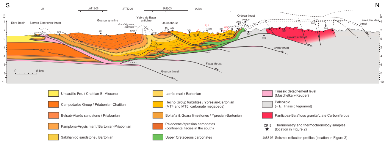
Figure 5. Balanced cross section of the eastern Jaca Basin (see Figure 2 for location). Surface data were compiled from published maps [Puigdefábregas Tomás, 1975; Gil Peña et al., 1990; Rios Aragües et al., 1990; Montes Santiago, 1991; Ternet et al., 2003; Millán Garrido, 2006], complemented with own field observations. Subsurface structures are derived from the seismic interpretation shown in Figure 6. Seismic profiles and projected thermometry and apatite fission track samples are located in Figure 2.
