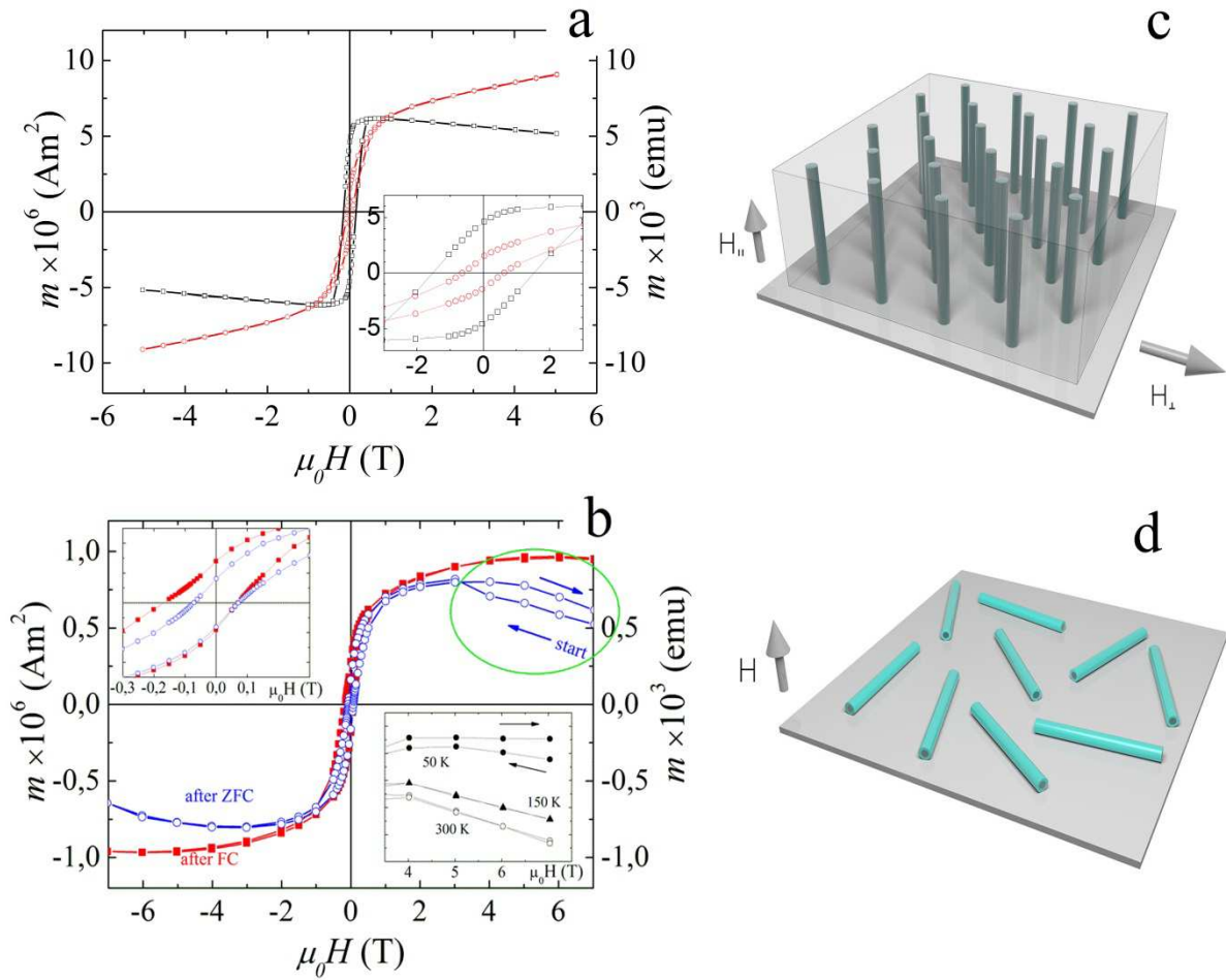
Figure 2. (a) Hysteresis loops of the aligned cobalt wires embedded in the anodised alumina membrane measured at 10 K (after field cooling) parallel (—□—) and perpendicular (—○—) to the nanowire axis, respectively. (b) Out-of-plane hysteresis loops for free-standing of Co|CoO core-shell nanowires traced at 10 K starting from +7 T after either ZFC (—○—) or FC in 5 T (—■—) from 300 K. The top inset shows a magnification of the low field region of the loops. The bottom inset shows the high field magnetization measured at 50, 150 and 300 K, after ZFC. No diamagnetic correction has been performed to any of the loops. The lines are guides to the eye. The ellipse in (b) highlights the high-field irreversibility. Panels (c) and (d) show schematically the direction of the measuring field and the arrangement of the wires for the ones embedded in the alumina template and for the free-standing ones deposited on a Colodion membrane, respectively.
