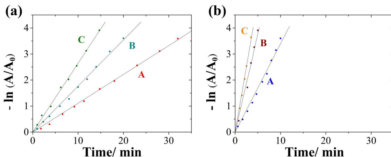
Figure 6: Plots of -\ln(A/A_0) against reaction time for the catalysed reduction of 4-NP by (a) compact and (b) mesoporous NWs in silent (A), intermittent ultrasound stirring (B) and magnetic stirring (C) conditions.
