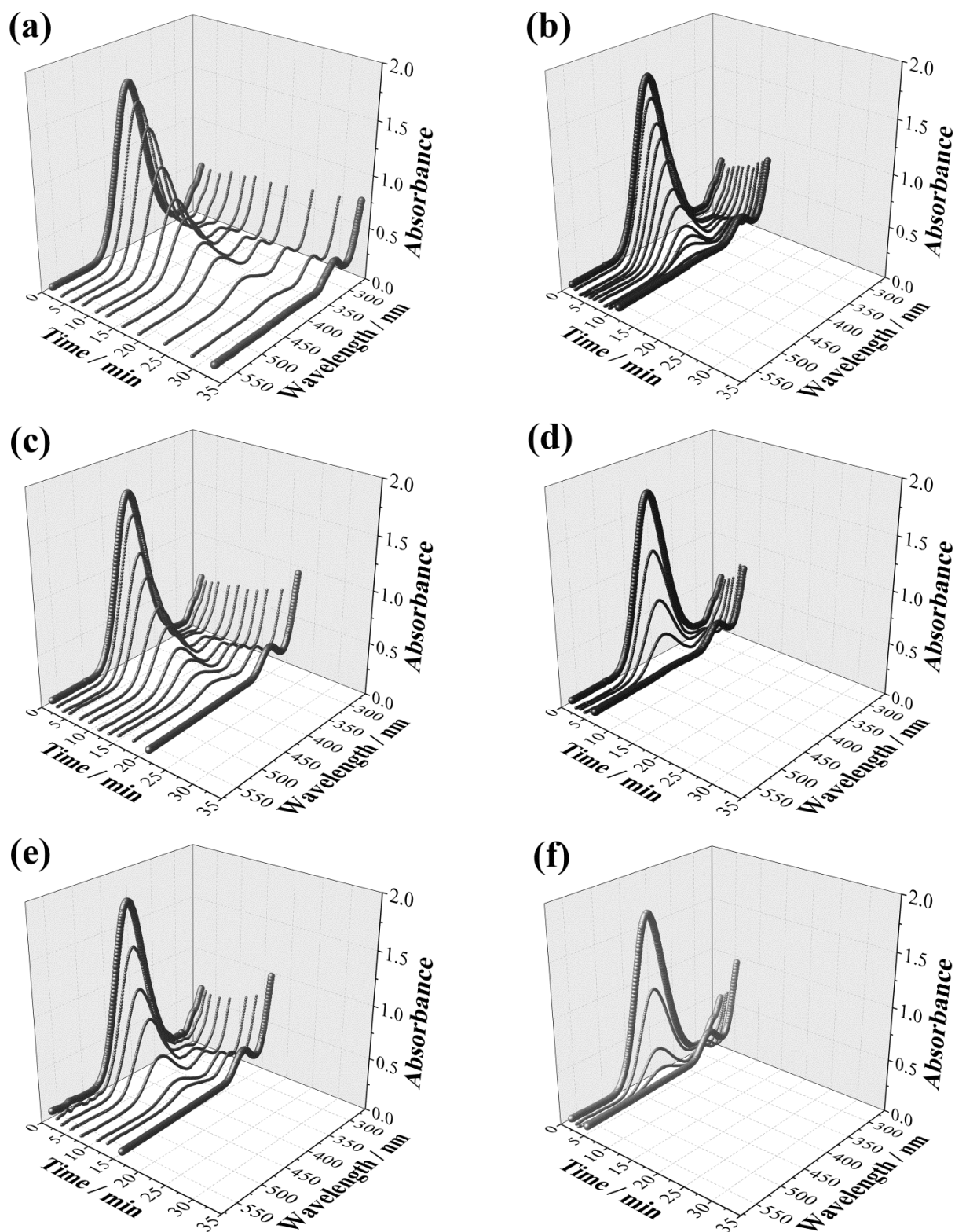
Figure 5: Time-dependent UV-Visible spectra of 4-NP catalyzed reduction in silent (panels a and b, for compact and mesoporous NWs, respectively), intermittent ultrasound stirring (panels c and d, for compact and mesoporous NWs, respectively) and magnetic stirring (panels e and f, for compact and mesoporous NWs, respectively) conditions, in which 12 \mu\text{L} of a suspension of catalyst ( 0.1 \text{ mg mL}^{-1} ) were added.
