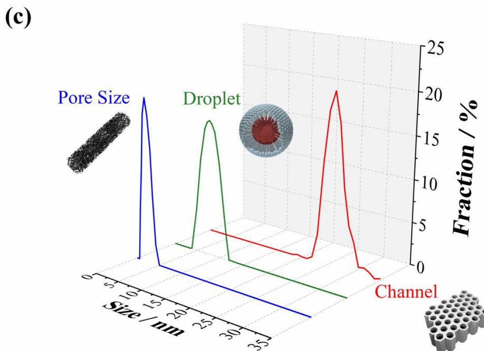
Figure 2: TEM images of the surface of (a) compact and (b) mesoporous magnetic Co–Pt NWs with diameters of 25 nm. Scale bar: 10 nm. (c) Size distributions of mesopores, droplets of ionic liquid and channels of alumina membrane.
