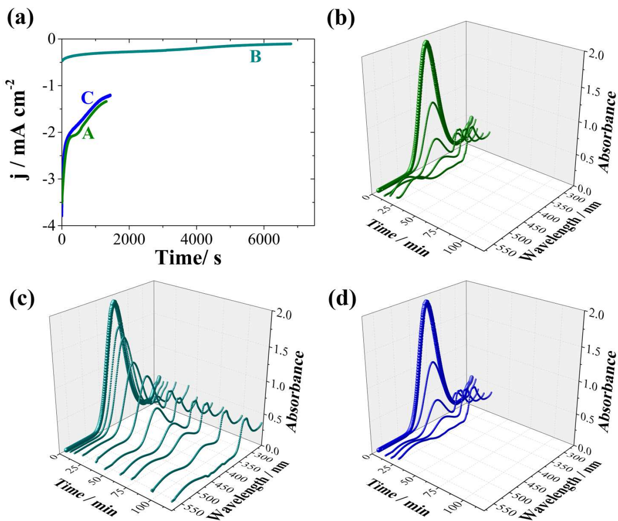
Figure 3: (a) Chronoamperometric curves (recorded at -0.35 V vs Ag/AgCl/KCl (3M)/H 2 SO 4 (0.5M)) of (A) Pt mesoporous, (B) Co-Pt compact and (C) Co-Pt mesoporous NWs for the electro-reduction of 4-nitrophenol. Time-dependent UV-Visible spectra of 4-NP electro-catalysed reduction using (b) Pt mesoporous, (c) Co-Pt compact and (d) Co-Pt mesoporous NWs.
