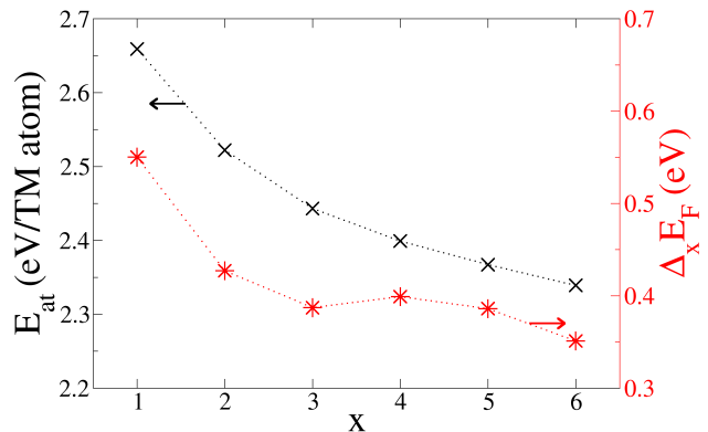
FIG. 3. Atomization energy, E_{at} from Eq. (3), (black x's) and the gain in energy by adding one more Mn atom the chain, \Delta_x E_F from Eq. (4), (red stars). As we can see, atomization of the chain becomes less difficult as the chain becomes longer, and correspondingly, adding one more atom does not reduce the total energy as much for longer chains. These values reveal an increasing destabilization of the chain as it size increases. The dotted lines are a guide for the eye.
