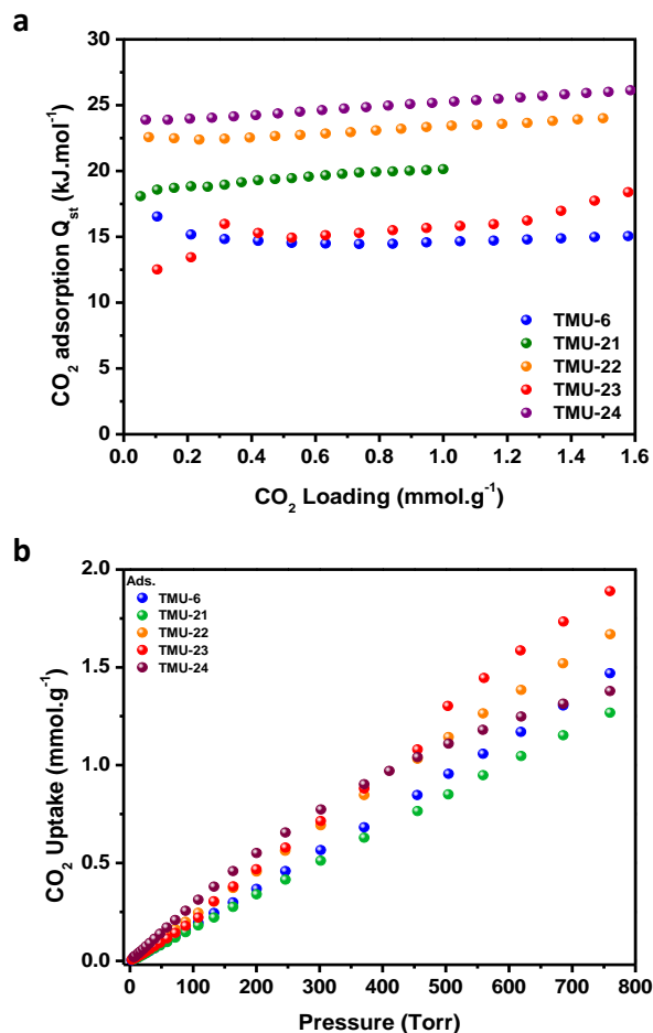
Figure 3. (a) Heats of adsorption of CO 2 and (b) CO 2 sorption isotherms at 298 K for TMUs-6/-21-24.
