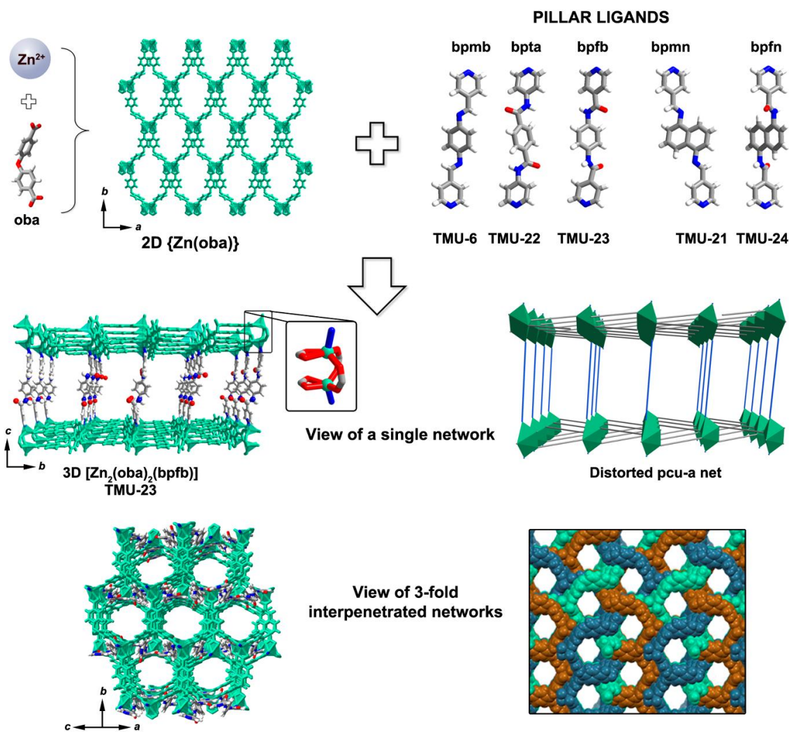
Figure 1. 2D layers formed by the association between Zn(II) ions and oba linkers are further pillared by amide/imine-functionalized dipyriddy-based ligands yielding to 3D-interpenetrated porous pcu -MOFs.
