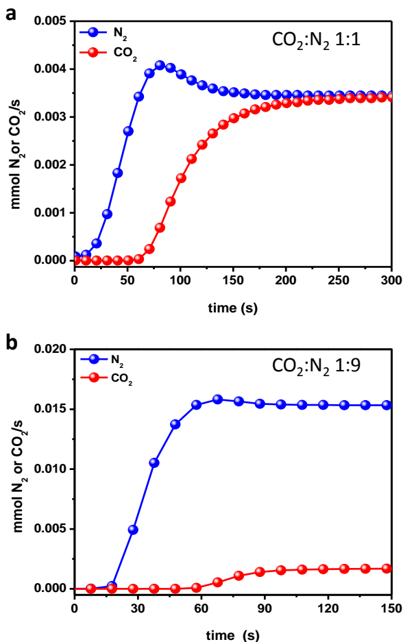
Figure 5. CO 2 /N 2 Breakthrough separation curves at 298 K for TMU-24 with total flow of 5 mL.min -1 for CO 2 :N 2 = 1:1 (a) and 25 mL.min -1 for 1:9 (b).
