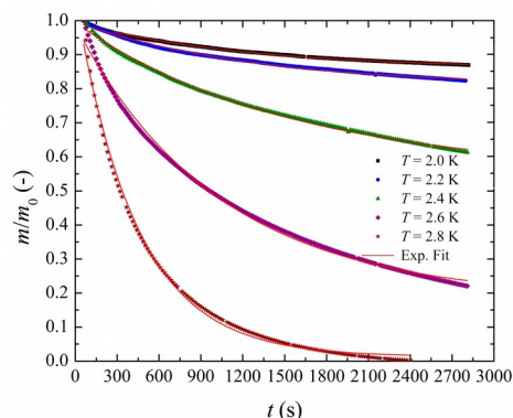
Figure 3. Exponential time relaxation of the normalized magnetization in a field of -20 Oe at different temperatures from 2.0 K to 2.8 K in increments of 0.2 K. become superparamagnetic. The absence of any secondary maxima in the ZFC curve indicates the presence of only one species of Mn 12 acetate having fixed magnetic anisotropy energy of about 65 K. Hysteresis loops of the magnetization taken at different temperatures are shown in Figure 2a. The corresponding descending branches are obtained by first saturating Mn 12 _triclinic in a positive magnetic field of up to 3 T, and then reducing the magnetic field to zero, reversing it, and increasing the field in the opposite direction at a constant rate. Analogous protocol is carried out for the ascending branches. Striking feature of these magnetization curves is a very large narrow jump of the magnetization at zero field for both ascending and descending protocols. In the past, such jumps have only been seen in a large magnetic field due to the phenomenon of magnetic deflagration. 8,9 The latter is equivalent to chemical combustion: reversal of the magnetic moments of the molecules leads to the release of their Zeeman energy into heat that further enhances magnetic relaxation. However, at B = 0 , there is no Zeeman energy to burn, so that the deflagration as an explanation to the jumps is ruled out. The derivative of the normalized magnetization, d(M/M_s)/dH , along the descending branch is shown at different temperatures in Figure 2b. It clearly indicates four tunneling maxima at the conventional resonant fields of Mn 12 acetate, separated by about 0.46 T. Analogous behavior is observed for the ascending protocol. The presence of such maxima in d(M/M_s)/dH of non-oriented amorphous particles of a molecular magnet has been explained in a previous study. 18 The new feature is an extremely narrow width of the zero-field maximum. In some instances, it is below 50 Oe (Figure 2b, inset). Such a narrow spin tunneling resonance has never been observed in any molecular magnet.
