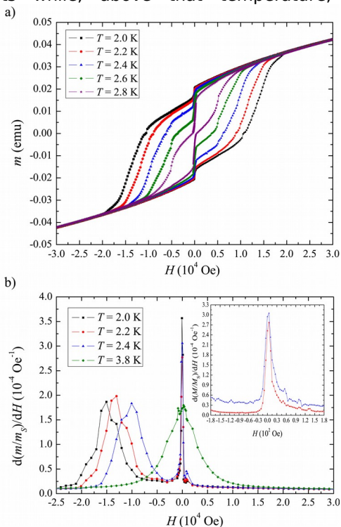
Figure 2. a) Hysteresis loops of the magnetization of Mn 12 _triclinic taken at different temperatures. The data along the descending branch is obtained by saturating the sample in a positive field and reducing and reversing the magnetic field. The curves show large jumps at zero field that have not been previously observed in Mn 12 Lis phase. b) d(M/M_s)/dH along the descending branch of Mn 12 _triclinic at different temperatures. Spin-tunneling maxima at zero and first resonant fields are clearly observed. Inset shows low field structure of the zero field maximum at 2.2 and
