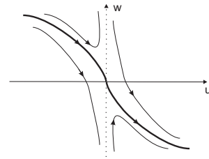
FIGURE 8. Phase portrait of system (14). The vertical axis is filled of singular points.
