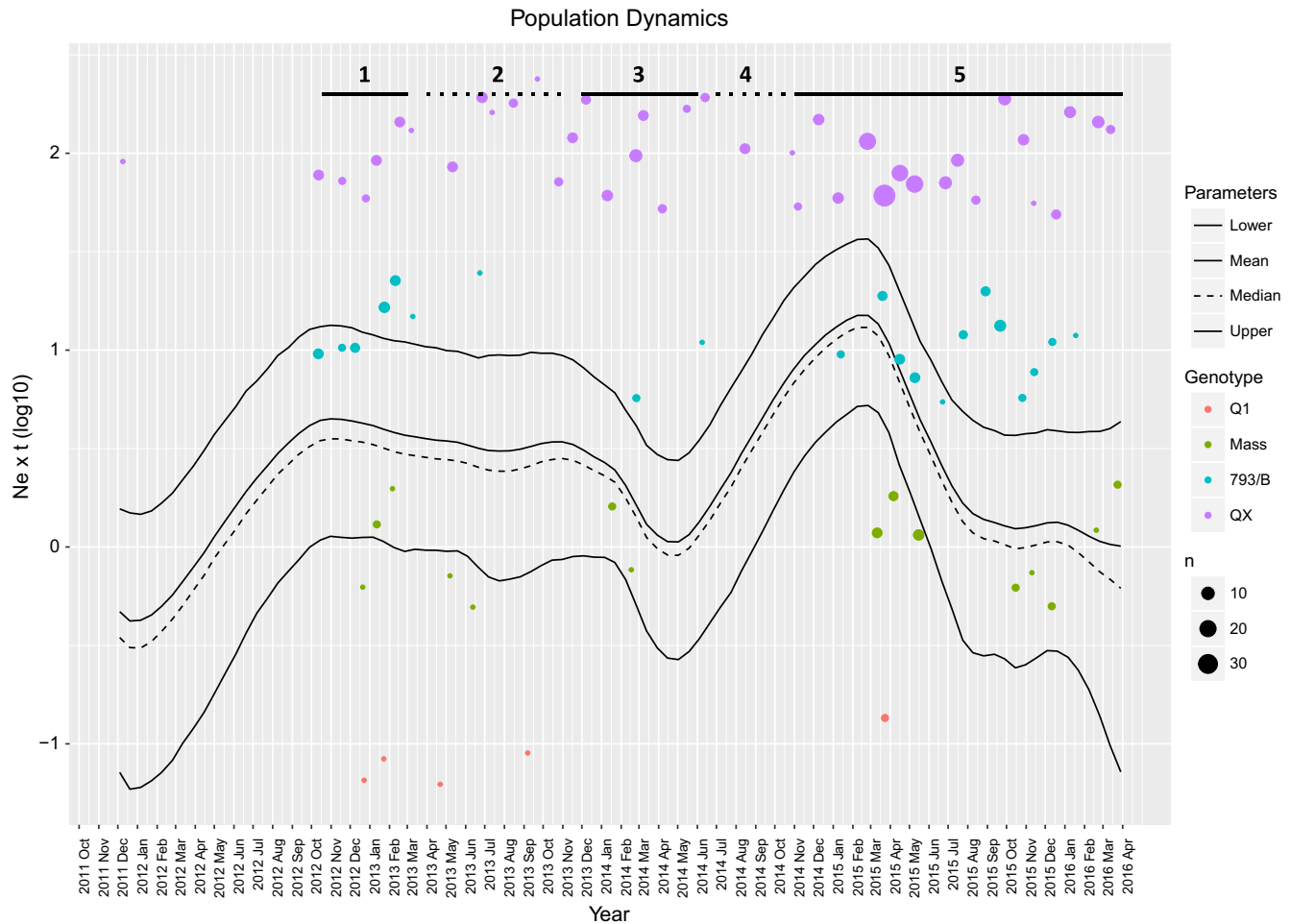
Fig. 2. Bayesian skyline plot of population dynamics estimated for Italian IBV QX strains. Mean, median and upper and lower 95HPD values of relative genetic diversity (i.e. N_e \cdot t ) are plotted over time. The number of monthly clinical outbreaks associated to each genotype (color-coded) is reported as circles (randomly jittered to avoid graphical overlapping), whose radius is proportional to the number of events. The different phases (i.e. vaccination strategies) have been represented as solid (double vaccination) or dotted (Mass only vaccination) lines and numbered accordingly to the order reported in the manuscript. The time window considered ranges from the MRCA (mean value) to the most recent sample. (For interpretation of the references to colour in this figure legend, the reader is referred to the web version of this article.)
