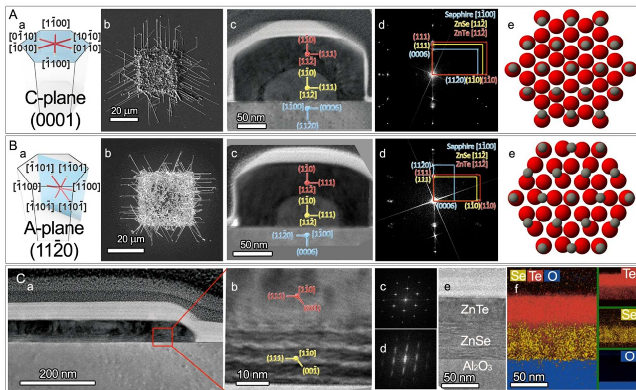
Figure 2. Guided growth of epitaxial core-shell nanowires on C-plane and A-plane sapphire. (A-B) For each substrate: (a) A schematic illustration of the plane and directional growth. (b) SEM image of the guided Nanowires. (c) HRTEM cross-section image, marked with the crystal planes and direction of the nanowire ZnSe core (yellow), ZnTe shell (red) and the sapphire substrate (blue). (d) Selected area fast Fourier transform (FFT) of the cross section image. (e) Top view of the atomic crystal structure, of only the topmost unit cell of sapphire and the lowest ZnSe core unit cell. (C) Analysis along a guided nanowire on A-plane sapphire: (a) HRTEM cross-section image. (b) Larger magnification of the indicated area marked with the crystal planes and direction of the nanowire ZnSe core (yellow), ZnTe shell (red). Selected area fast Fourier transform (FFT) of (c) the ZnTe shell and (d) the ZnSe core. EFTEM analysis with (e) zero loss image and (f) an elemental map overlay and the Se, Te, and O elemental maps.
