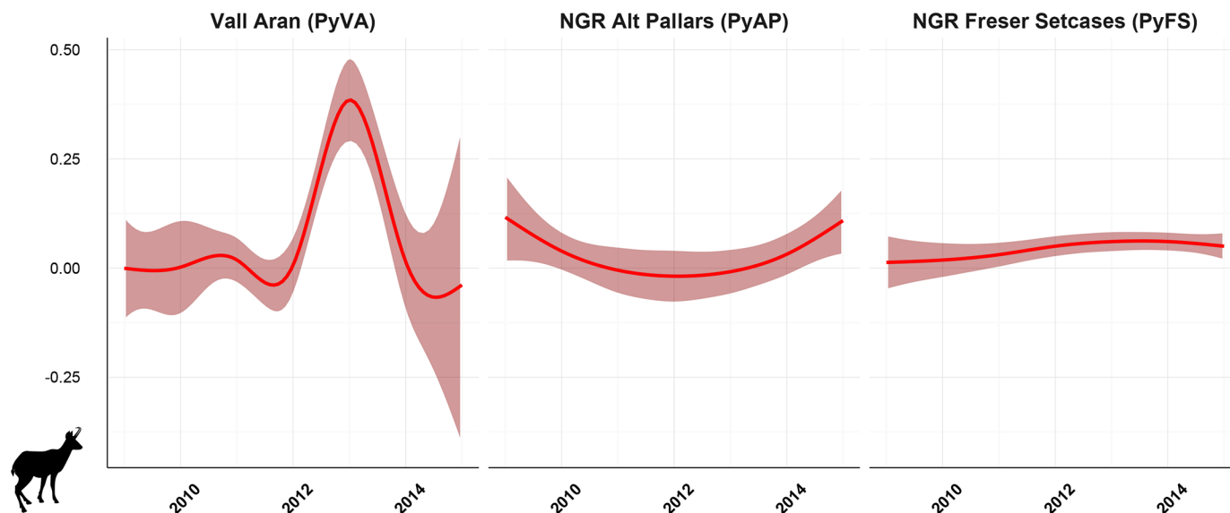
Fig 2. Modeled trend curves of Mycoplasma conjunctivae infection in Pyrenean chamois by generalized additive models. Infection indices show evident curve differences by study area, in which the interaction of year with the study area resulted statistically significant in NGR Alt Pallars and Vall Aran, but not in NGR Freser Setcases.
