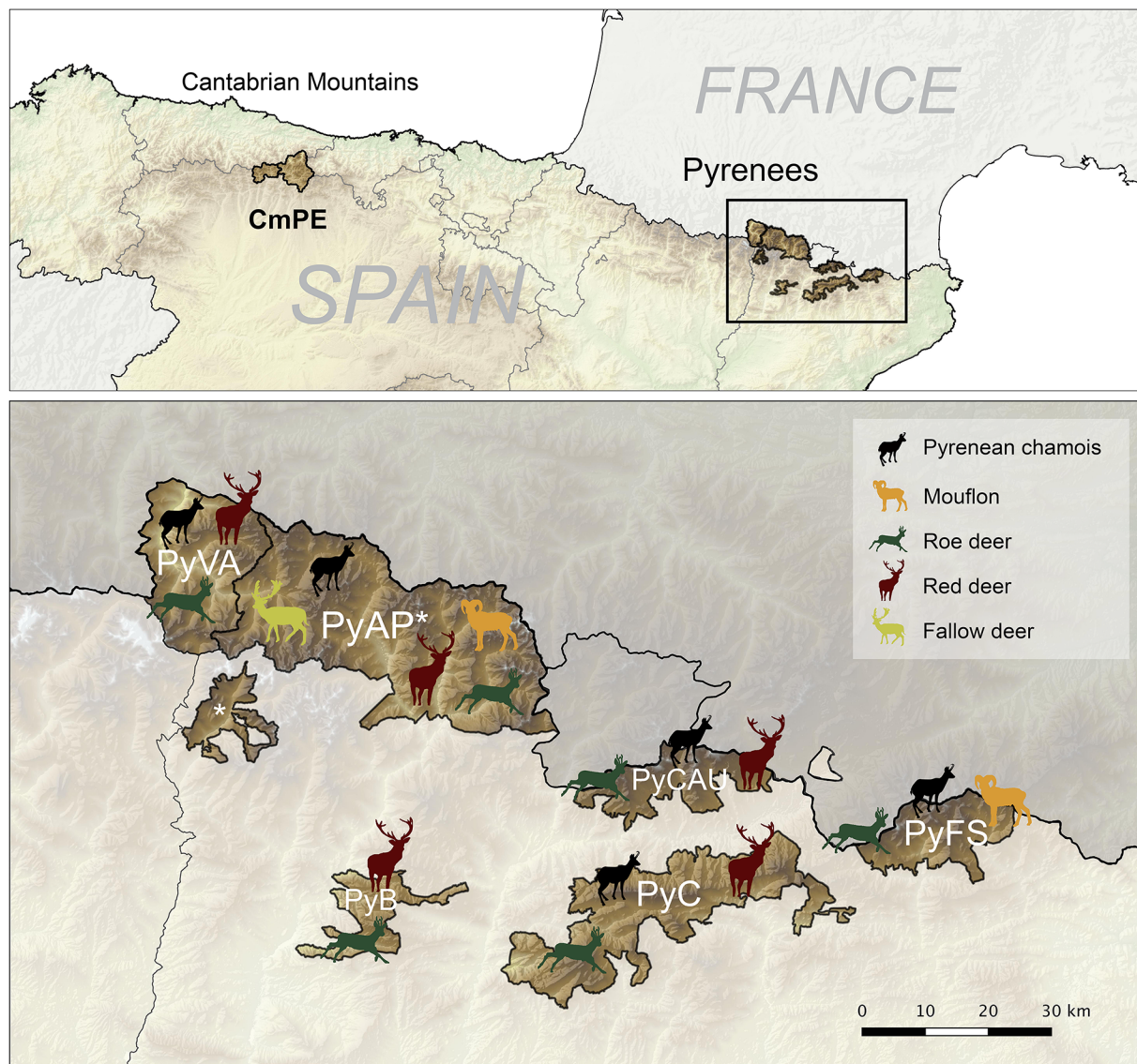
Fig 1. Maps of the study areas and wild ruminant species composition in the Pyrenees. Location of the study areas in Cantabrian Mountains (Picos de Europa—CmPE) and Eastern and Central Spanish Pyrenees. Wild ruminant species composition by study area from the Pyrenees is showed in detail in the image of the bottom: Vall Aran (PyVA), NGR Alt Pallars (PyAP), NGR Boumort (PyB), NGR Cerdanya-Alt Urgell (PyCAU), NGR Cadí (PyC) and NGR Freser-Setcases (PyFS). The asterisk means the same study area. Chamois in PyB is scarce and not representative of the area (not shown in the map).
