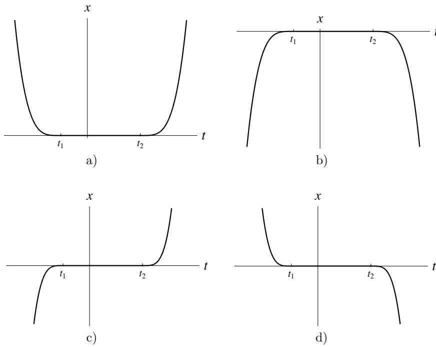
Figure 3: Examples of solutions of (1) with \varphi(t) = (0, 0) for some t \in \mathbb{R} . a) Solution with x(t) > 0, y(t) < 0 for t < t_1 , x(t) = 0, y(t) = 0 for t \in [t_1, t_2] , and x(t) > 0, y(t) > 0 for t > t_2 . b) Solution with x(t) < 0, y(t) > 0 for t < t_1 , x(t) = 0, y(t) = 0 for t \in [t_1, t_2] , and x(t) < 0, y(t) < 0 for t > t_2 . c) Solution with x(t) < 0, y(t) > 0 for t < t_1 , x(t) = 0, y(t) = 0 for t \in [t_1, t_2] , and x(t) > 0, y(t) > 0 for t > t_2 . d) Solution with x(t) > 0, y(t) < 0 for t < t_1 , x(t) = 0, y(t) = 0 for t \in [t_1, t_2] , and x(t) < 0, y(t) < 0 for t > t_2 .
