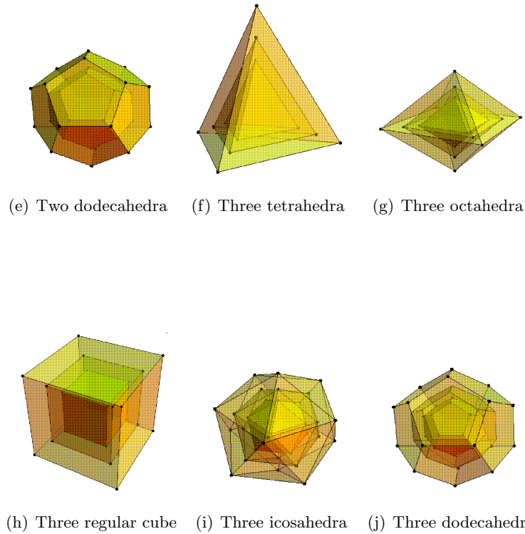
FIGURE 1. Nested regular polyhedra, with two or three polyhedra.
