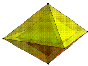
(b) Two octahedra
