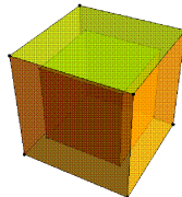
(c) Two cube
