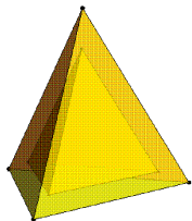
(a) Two tetraedra
