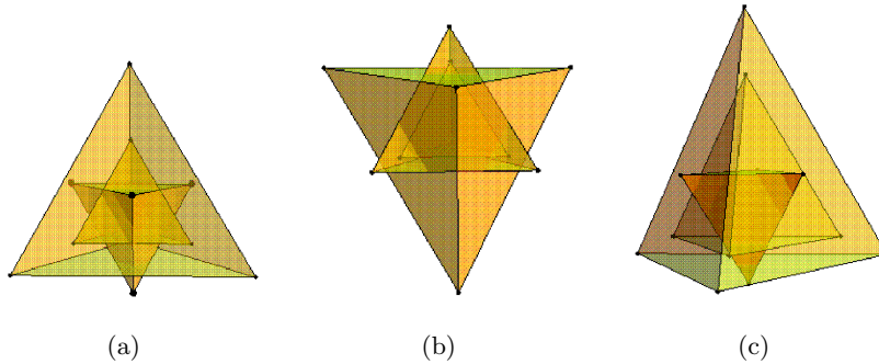
FIGURE 2. Three rotated tetrahedra.
