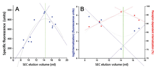
Fig. 5 Relationships between relevant parameters of T22-GFP-H6 nanoparticle populations. A. Regression lines for specific fluorescence F(E) (blue), quadratic prediction F(E) (grey), and symmetry point (green). B. Regression curves for protein internalization (logarithm) I(E) (blue) and receptor-dependent cell internalization R(E) (red) in terms of the SEC-elution volume. Quadratic predictions in grey and symmetry point in green.
