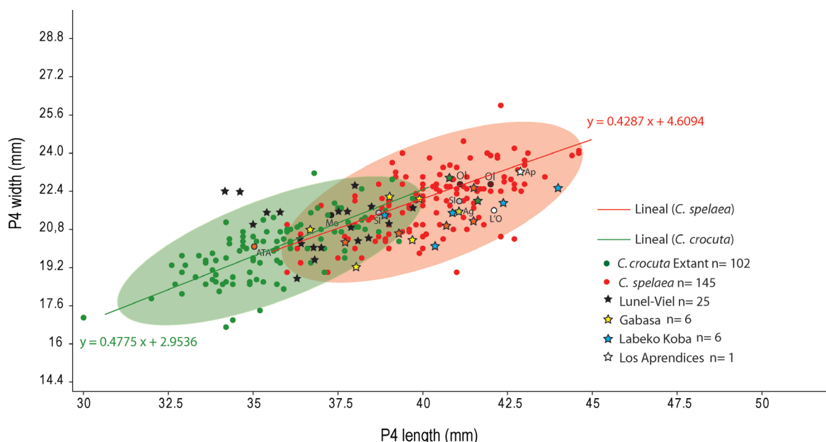
FIGURE 9. Graph representing total length versus total width of P4 of extant and cave hyaena from several sites. The comparative measurements have been extracted from, Reynolds, 1902; Bonifay, 1971; Ballésio, 1979; Clot, 1980; Argant, 1991; Cardoso, 1993; Blasco and Montes, 1997; Fosse, 1997; Castaños, 1987; Baryshnikov, 1999; Altuna and Mariezkurrena, 2000; García, 2003; Testu, 2006; Fourvel, 2012; and J.M.-M personal commun., 2015. Abbreviations: ATA, Atapuerca; Ag, Aguilón P-7; Ap, Los Apendices; Mo, Mollet; OL, Olopte B; L'Or Cova de l'Or; SI, Sima I. Confidence ellipses with confidence interval (0.95) are figured.
