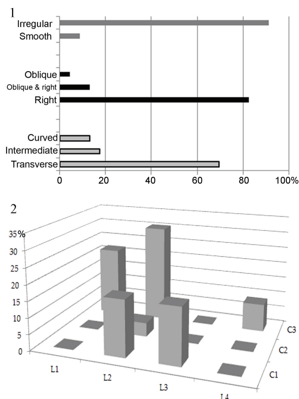
FIGURE 13. 1, Analysis of the breakage of the long bones from the skeleton of Crocutea spelaea from Los Apendices, showing the abundance of each type of fracture according to the criteria analysed: angle, delineation and edge of the breaks. 2, Analysis of the breakage of the diaphyses in terms of circumference (C1, C2, C3) and length (L1, L2, L3, L4) for the skeleton of Crocutea spelaea from Los Apendices.
