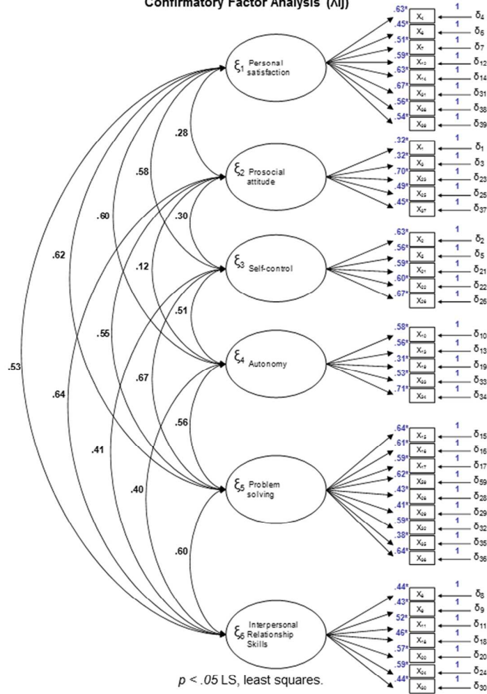
Figure 1: Factor loadings derived from the LS estimation (least squares) Confirmatory Factor Analysis ( \lambda_{ij} )
