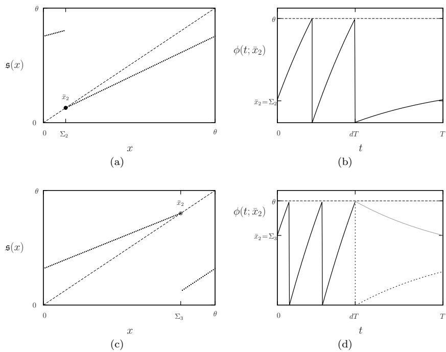
Figure 7.18: (a) Fixed point \bar{x}_2 colliding with the boundary \Sigma_2 for A = A_2^{\mathcal{R}} (b) T -periodic orbit for A = A_2^{\mathcal{R}} . (c) fixed point \bar{x}_2 colliding with the boundary \Sigma_3 for A = A_3^{\mathcal{L}} . (d) T -periodic orbit for A = A_3^{\mathcal{L}} . Note that the periodic orbit in (d) should exhibit a reset at t = dT ; this is why it is plot in gray color.
