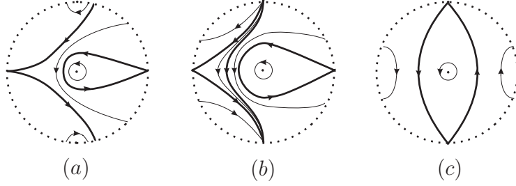
FIGURE 1. Phase portraits of uniform isochronous cubic centers.
