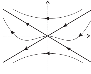
FIGURE 3. Correct local phase portrait corresponding to Figure 20 of [6].
