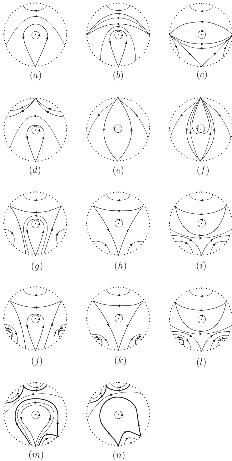
FIGURE 2. Phase portraits of uniform isochronous quartic centers.
