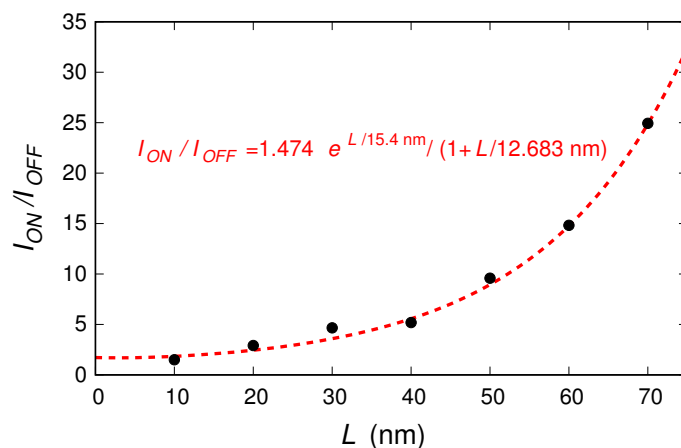
Figure 5. The black dots show the values of the I_{ON}/I_{OFF} ratio obtained for the double-gate field-effect-transistor based on the graphene ribbon with a 0.6% boron concentration, for the seven considered ribbon lengths. The red dashed line represents the extrapolated analytical behavior.
