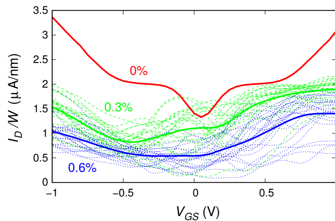
Figure 2. Transfer characteristics (obtained for V_{DS} = 0.1 V) of the double-gate field-effect-transistor based on a 20-nm-long graphene ribbon with a boron concentration of 0% (undoped ribbon), 0.3%, and 0.6%. The thin lines (dashed for the 0.3% boron concentration, dotted for the 0.6% boron concentration) show the results for 23 individual realizations of the dopant distribution, while the thick lines represent the average over the ensemble. The current value was divided by the ribbon width W = 3.81 nm in order to represent the current density.
