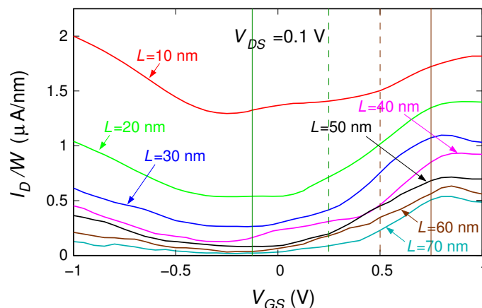
Figure 4. Average transfer characteristics (obtained for V_{DS} = 0.1 V) of the double-gate field-effect-transistor based on a graphene ribbon with a 0.6% boron concentration over a length of 10, 20, 30, 40, 50, 60, and 70 nm. The current value was divided by the ribbon width W = 3.81 nm in order to represent the current density. The four vertical lines identify the values of V_{GS} for which the values plotted in Figure 6 were extracted.
