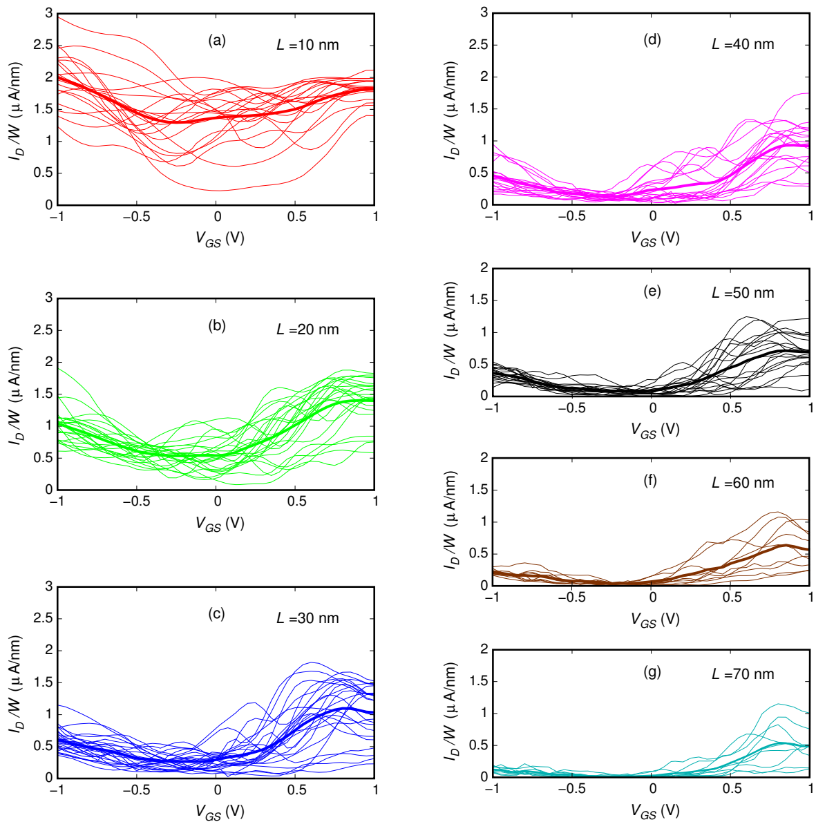
Figure 3. Transfer characteristics (obtained for V_{DS} = 0.1 V) of the double-gate field-effect-transistor based on a graphene ribbon with a 0.6% boron concentration over a length of (a) 10 nm, (b) 20 nm, (c) 30 nm, (d) 40 nm, (e) 50 nm, (f) 60 nm, and (g) 70 nm. The thin lines correspond to the individual realizations of the dopant distribution, while the thick lines correspond to the average. The current value was divided by the ribbon width W = 3.81 nm in order to represent the current density.
