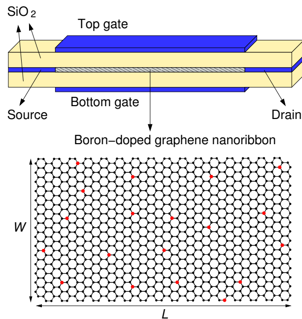
Figure 1. Sketch of the considered field-effect-transistors. The transmission channel is a boron-doped armchair graphene nanoribbon, represented at the bottom: black and red atoms are carbon and boron atoms, respectively, while the hydrogen atoms passivating the edges are not represented.
