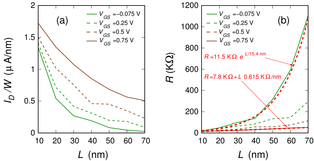
Figure 6. (a) Current density I_D/W (with W = 3.81 nm) and (b) Channel resistance R = V_{DS}/I_D as a function of the length L for the four values of the voltage V_{GS} identified by the vertical lines in Figure 4. In panel (b), the dashed red curves indicate the fit of the channel resistance as a function of the channel length for V_{GS} = -0.075 V and V_{GS} = 0.75 V, which we take as representative of the OFF state and ON state, respectively, based on the analytical formulas for localized and diffusive transport regimes.
