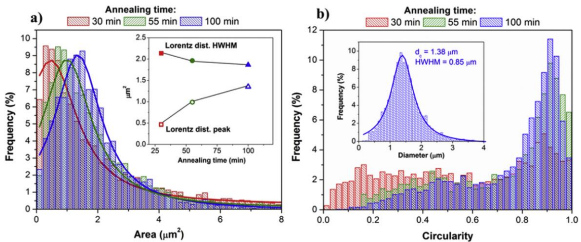
Fig. 2. a) Islands area distribution formed at TA \approx 870 ^{\circ} C and for different tA fitted with the corresponding Lorentz curve (solid line); inset: evolution of peak and HWHM of Lorentz curve as a function of tA. b) Islands circularity distribution formed at TA \approx 870 ^{\circ} C and for different tA; inset: islands diameter distribution formed at TA \approx 870 ^{\circ} C for tA \approx 100 min with the corresponding Lorentz curve (solid line).
