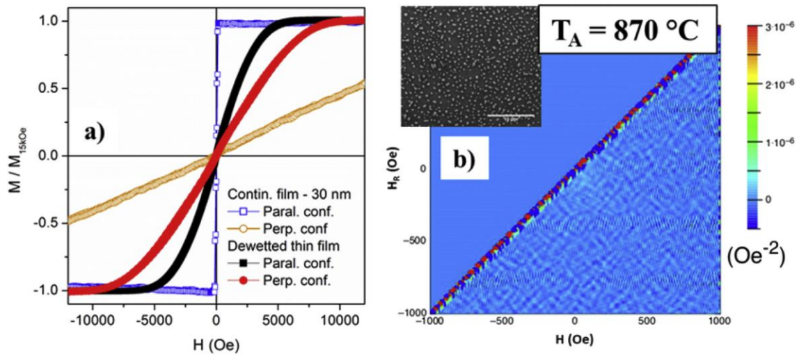
Fig. 5. a) normalized room-temperature hysteresis loops of FePd samples ( t \approx 30 nm) in as-deposited continuous state (blue and orange curve) and after dewetting at T_A \approx 870 °C for t_A \approx 55 min (red and black curve) measured both in-plane and out-of-plane configuration. b) FORC colour plot of sample dewetted at T_A \approx 870 °C for t_A \approx 55 min, inset: SEM image of the sample.
