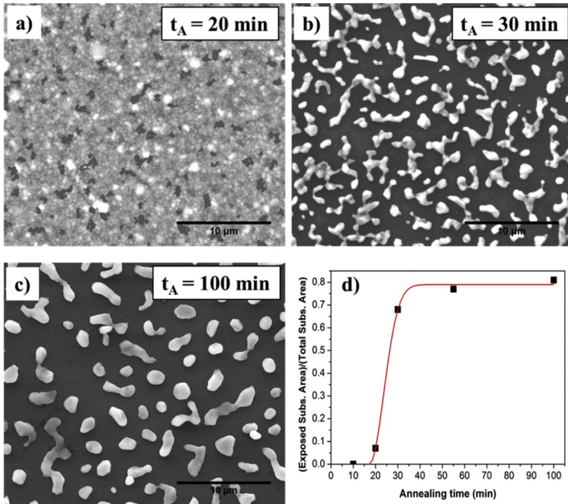
Fig. 1. a) e c) FePd thin film ( t \approx 100 nm) morphology after annealing at T_A \approx 870 °C for selected t_A : 20, 30 and 100 min; d) fraction of exposed substrate area as a function of t_A (black square) according to Johnson-Mehl-Avrami model (red line).
