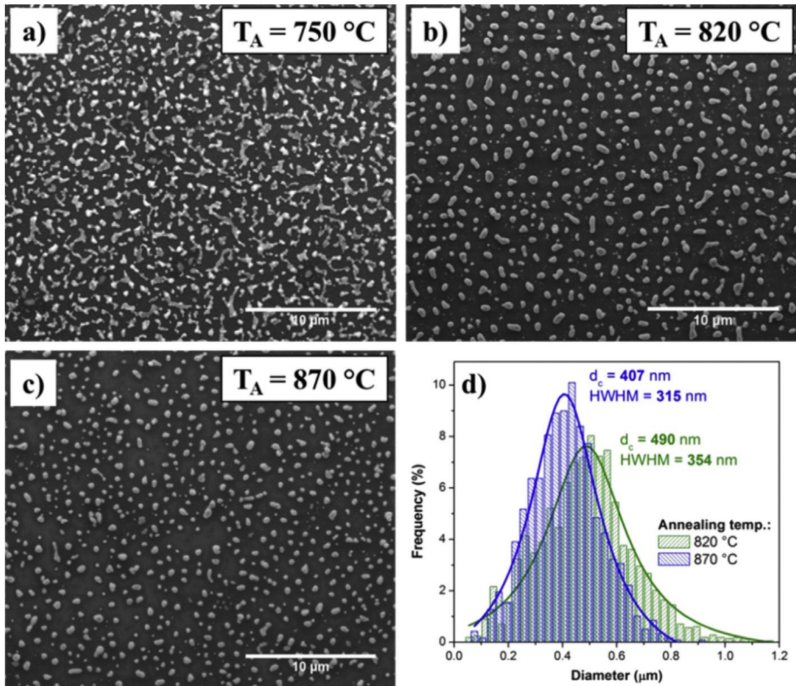
Fig. 3. a) c) FePd thin film ( t \approx 30 nm) morphology after annealing for t_A \approx 55 min at selected temperature ( T_A ): 750, 820, and 870 °C; d) islands diameter distribution of sample b) and c).
