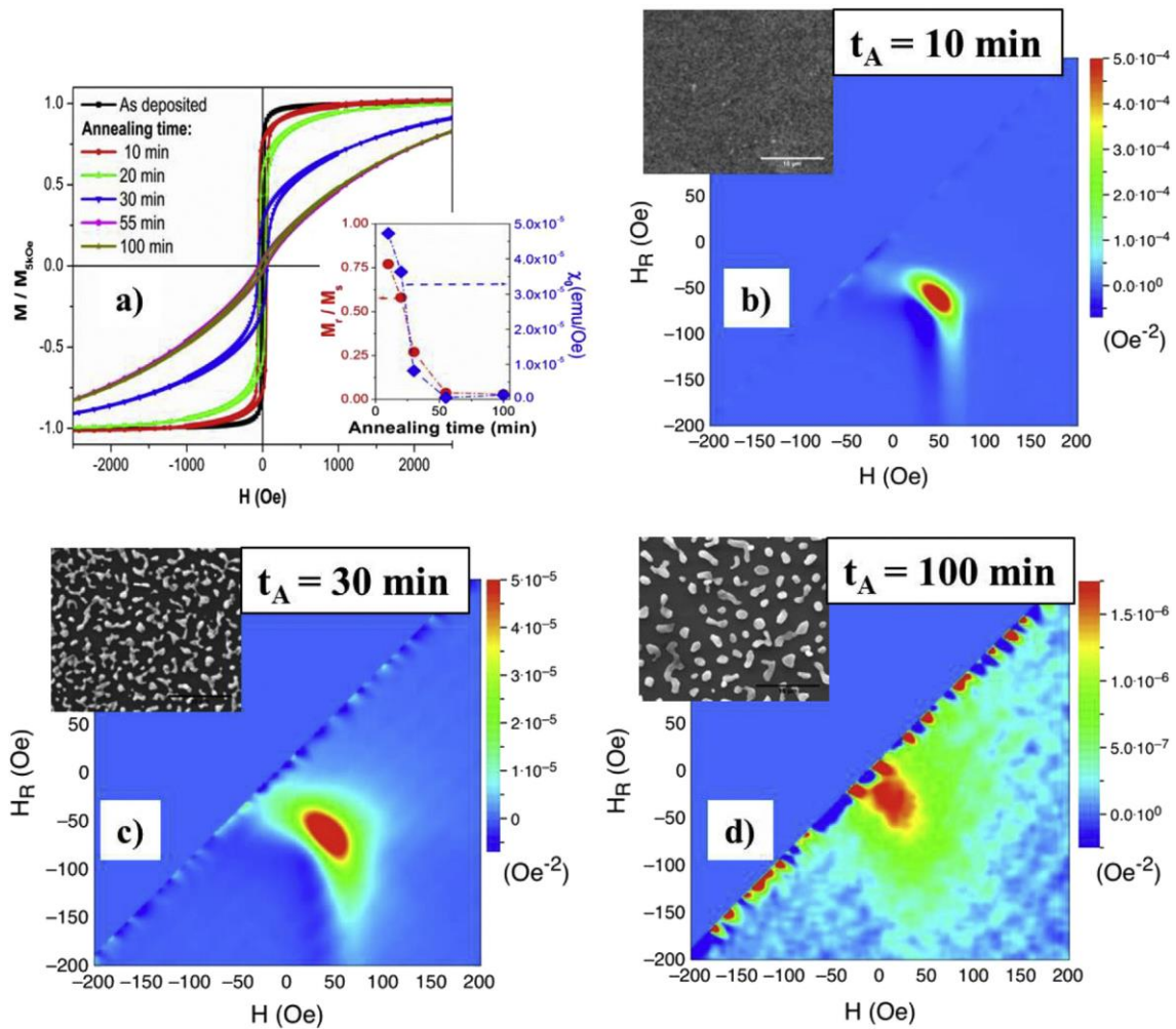
Fig. 4. a) Normalized room-temperature hysteresis loops of as-deposited and dewetted samples at T_A = 870 \text{ }^\circ\text{C} for selected t_A , inset: magnetization remanence and coercive susceptibility as a function of t_A ; b) - d) FORCs colour plot of dewetted samples at T_A = 870 \text{ }^\circ\text{C} for selected t_A , inset: SEM image of the corresponding sample.
