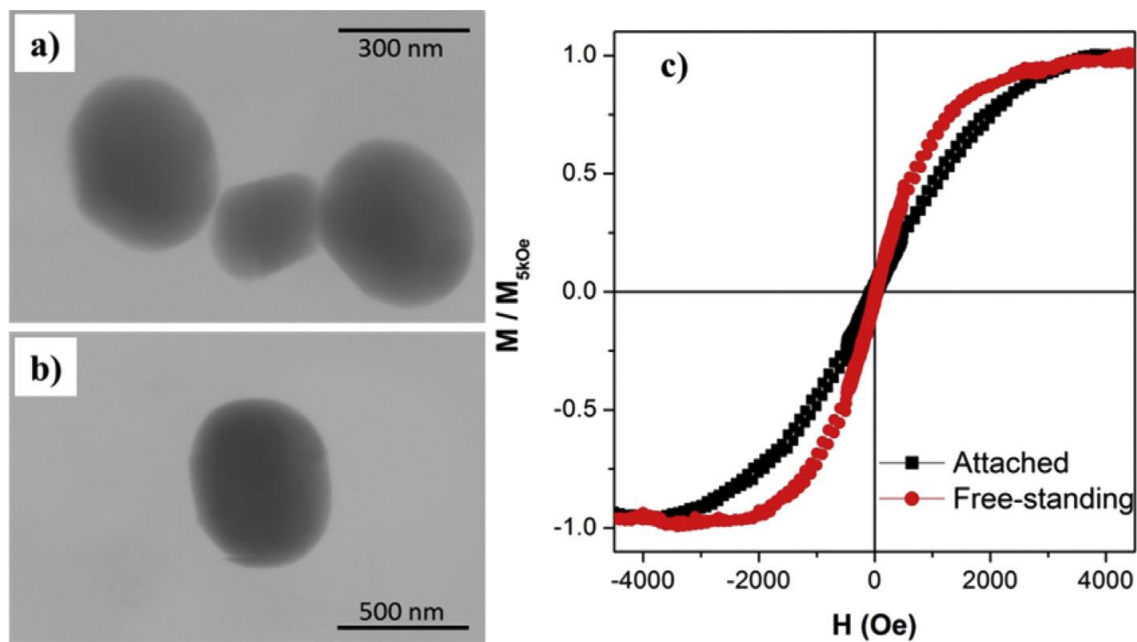
Fig. 6. a) - b) STEM images of free-standing FePd nanoparticles; c) normalized room-temperature hysteresis loops of FePd islands still attached on the substrate (black curve) and subsequently dispersed in acetone (red curve).
