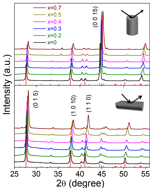
Figure 2. XRD patterns of consolidated \text{Bi}_2\text{Te}_{3-x}\text{Se}_x pellets measured in the two directions, parallel and normal to the pressing direction.
