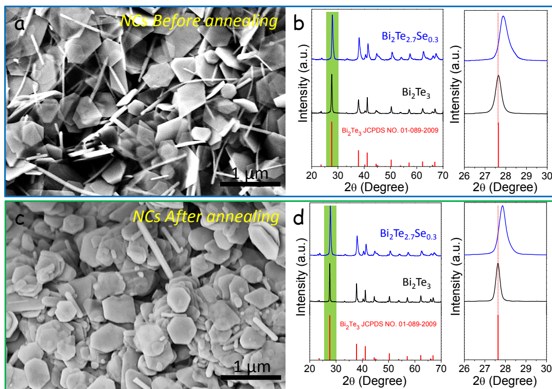
Figure 1. Representative SEM images (a, c) and XRD patterns (b, d) of the \text{Bi}_2\text{Te}_{3-x}\text{Se}_x disk-shaped NCs produced and used in this work, before (a, b) and after (c, d) annealing at 350^\circ\text{C} for 60 min. A detail of the same XRD pattern showing the shift of the (015) peak with the Se composition ( x=0, 0.3 ) is also provided. The standard \text{Bi}_2\text{Te}_3 diffraction pattern (JCPDS NO. 01-089-2009) is included as reference.
