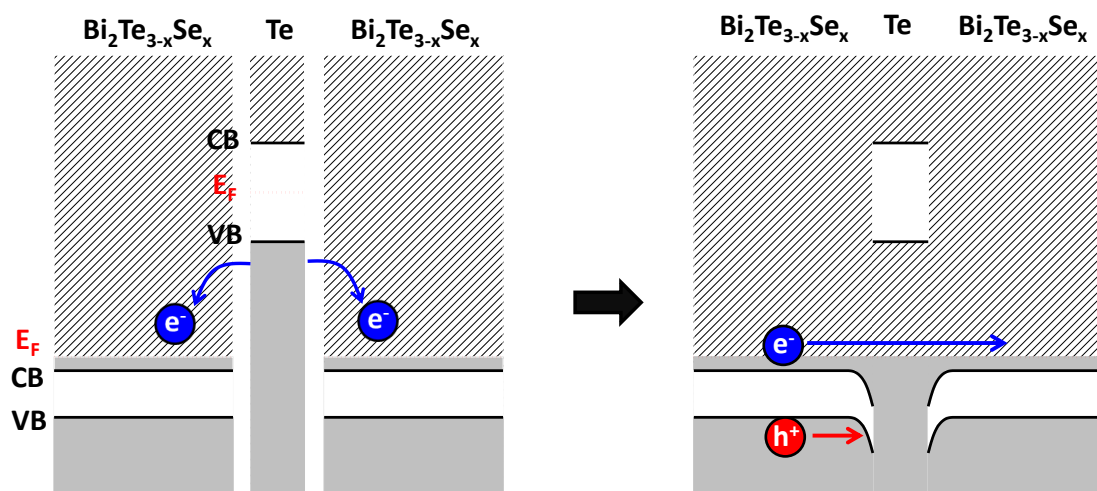
Figure 10. Scheme of the energy band alignment between Te ( \Phi = 4.7 \text{ eV} ; E_g = 0.33\text{-}0.36 \text{ eV} ) 58-60 and \text{Bi}_2\text{Te}_{3-x}\text{Se}_x ( \text{Bi}_2\text{Te}_3 : \Phi = 5.30 \text{ eV} ; E_g = 0.17 \text{ eV} ), 61, 62 underlying the charge injection from Te to \text{Bi}_2\text{Te}_{3-x}\text{Se}_x .
