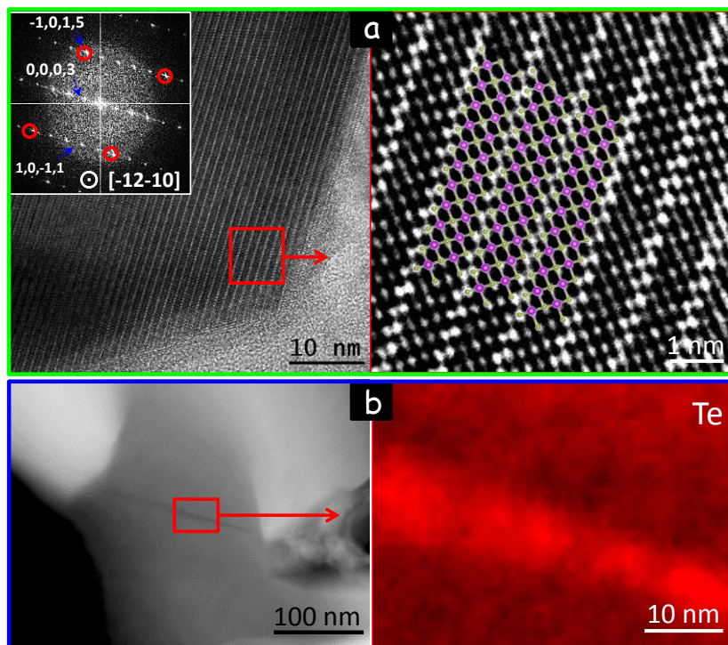
Figure 4. (a) HRTEM image of a \text{Bi}_2\text{Te}_{2.7}\text{Se}_{0.3} crystal within a consolidated pellet. The corresponding power spectrum, consistent with the [-12-10] zone axis of the \text{Bi}_2\text{Te}_{2.7}\text{Se}_{0.3} structure, is shown as an inset. Also shown (right) a detail of the squared region of the HRTEM image overlaid with the structure of \text{Bi}_2\text{Te}_{2.7}\text{Se}_{0.3} : Bi in purple, Se and Te in green, with partial occupations on the same sites. (b) ADF-STEM (left) and STEM-EELS Te composition map (right) of the interface of two crystals within the consolidated pellet, showing an excess of Te.
