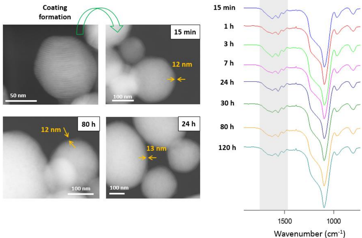
Figure 4. STEM images of MSN@pNDGA nanoparticles upon exposition to the PBS buffer at different time intervals. Coating thickness remains essentially unchanged (left). FT-IR spectra of MSN@pNDGA showing the persistence of the pNDGA coating upon exposition to the PBS buffer (right).
