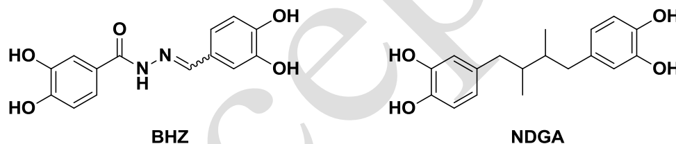
Scheme 1. Chemical structure of BHZ and NDGA bis-catechols.
