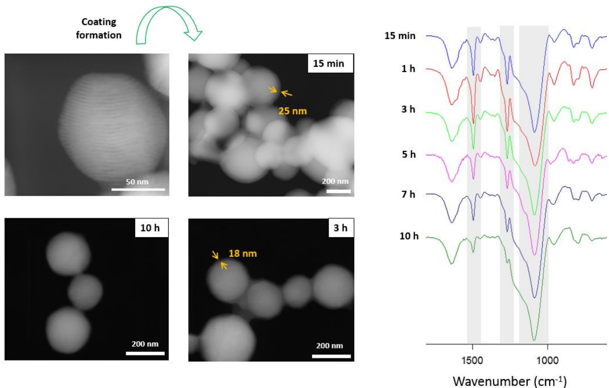
Figure 3. STEM images of MSN@pBHZ nanoparticles upon exposition to the PBS buffer at different time intervals. After 10 h, the coating cannot be observed any more (left). FT-IR spectra of MSN@pBHZ showing the progressive removal of the pBHZ coating upon exposition to the PBS buffer (right).
