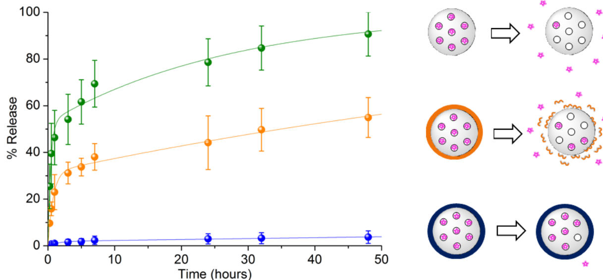
Figure 5. Experimental data corresponding to the release profiles of RhB from (●) RhB@MSNs, (●) RhB@MSN@pBHZ and (●) RhB@MSN@pNDGA and their corresponding model fitting curves for (—) RhB@MSNs, (—) RhB@MSN@pBHZ and (—) RhB@MSN@pNDGA.
