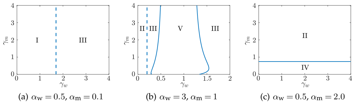
Figure 6. Two-dimensional bifurcation diagrams for \gamma_w versus \gamma_m at different sets of \alpha_i , with i = m, w . Parameter values are given by (3.14) and (a) \alpha_w = 0.5, \alpha_m = 0.1 ; (b) \alpha_w = 3, \alpha_m = 1 ; and (c) \alpha_w = 0.5, \alpha_m = 2 . Dashed and solid lines correspond to transcritical and Hopf bifurcations, respectively. Region I: stability of trivial solution; Region II: stability of wt-free state; Region III: stability of coexistence state; Region IV: stable periodic orbit (PO) around the wt-free state; Region V: stable PO around the coexistence state.
