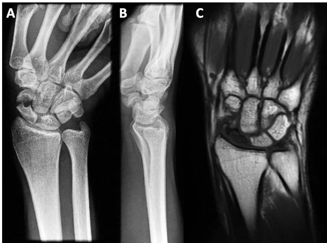
FIGURE 3 (A) Anteroposterior and (B) lateral radiographs and (C) a coronal MR image at four years of follow-up, showing recalcitrant nonunion and avascular necrosis of the scaphoid
