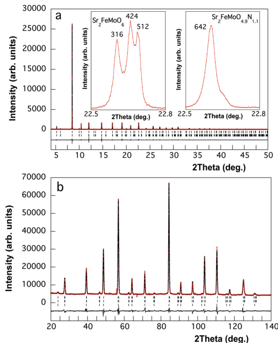
Fig. 2 Rietveld fits to (a) synchrotron X-ray powder diffraction pattern ( \lambda = 0.41269 \text{ \AA} ) and (b) neutron powder diffraction pattern ( \lambda = 1.86502 \text{ \AA} ) of \text{Sr}_2\text{FeMoO}_{4.9}\text{N}_{1.1} at 90 K. In (a) upper and lower ticks mark the reflections of Fm\bar{3}m \text{Sr}_2\text{FeMoO}_{4.9}\text{N}_{1.1} and I4/m SFMO impurity, respectively. In (b) the two upper ticks mark the nuclear and magnetic reflections of SFMO and the lower tick represents the nuclear reflections of \text{Sr}_2\text{FeMoO}_{4.9}\text{N}_{1.1} . The insets in (a) show selected regions to illustrate the symmetry change in the oxynitride with respect to the oxide. The small shoulder at the high 2\theta side of the 642 reflection corresponds to SFMO (refined fraction: 10.2(2)%).
