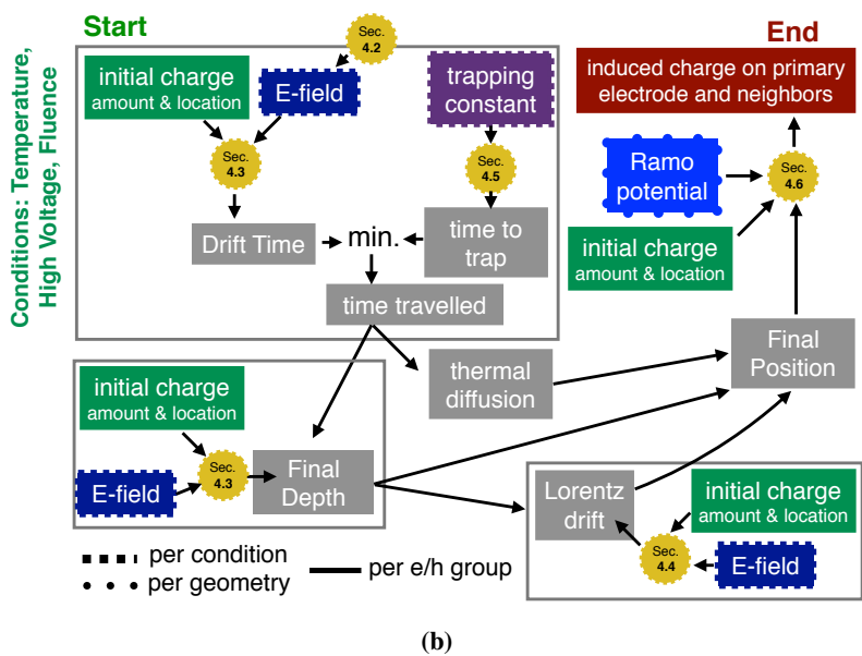
Figure 5. (a) A schematic diagram of the digitizer physics. As a MIP traverses the sensor, electrons and holes are created and transported to the electrodes under the influence of electric and magnetic fields. Electrons and holes may be trapped before reaching the electrodes, but still induce a charge on the primary and neighbour electrodes. (b) A flowchart illustrating the components of the digitizer model described in this article. The digitizer takes advantage of pre-computation to re-use as many calculations as possible. For example, many inputs are the same for a given condition (temperature, bias voltage, fluence). The Ramo potential [40, 41] only depends on the sensor geometry and the quantities in dashed boxes further depend only on the condition information (see also section 4.6). The output of the algorithm described in this paper is an induced charge on the primary electrode and the neighbours, which is then converted into a ToT by the existing software.
