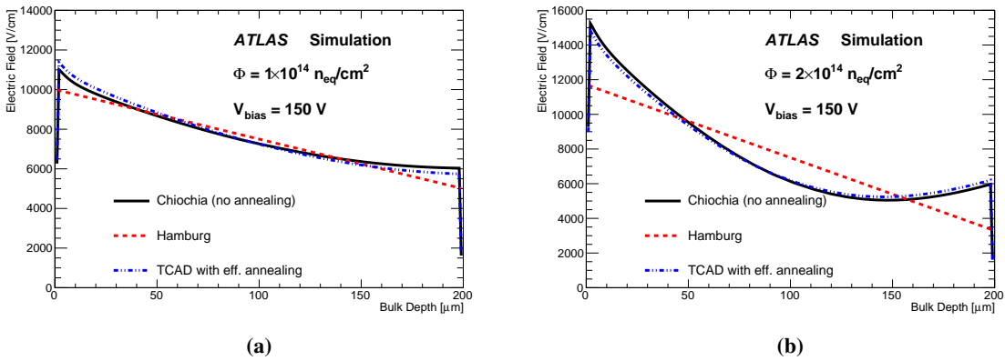
Figure 10. The z dependence of the electric field in a simulated ATLAS IBL planar sensor, averaged over x and y , for simulated fluences of (a) \Phi = 1 \times 10^{14} n_{\text{eq}}/\text{cm}^2 and (b) 2 \times 10^{14} n_{\text{eq}}/\text{cm}^2 . The bias voltage was set to 150 V in all cases. Three scenarios — Chiochia (no annealing), Hamburg and TCAD with effective annealing — to emulate annealing effects were simulated.
