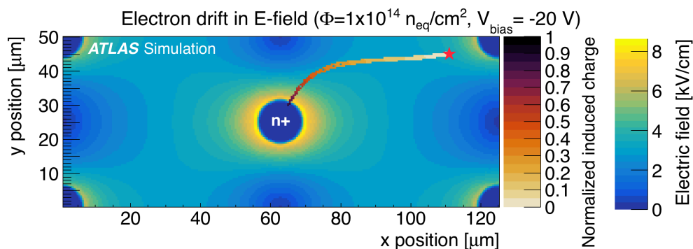
Figure 20. An illustration of charge trapping and the Ramo potential in one-half of a 3D sensor. The initial electrons originate from the top right corner of the plot (indicated by a star). Under the influence of the electric field, they drift toward the n^+ electrode in the centre. As they drift, there is a chance that they get trapped. Markers indicate the location of trapped charges and the colour shows the induced charge. The process is repeated many times, with diffusion. The simulated bias voltage was -20 V.
