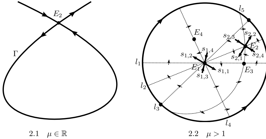
FIGURE 2. 2.1. The homoclinic loop of the saddle E_2 . 2.2. Local dynamics of the finite equilibria of systems (1) for \mu > 1 . l_1, l_2, l_4 are the straight lines through the equilibria E_1 and E_3, E_2, E_4 , respectively. l_3 is the straight line y = x . l_5 is the straight line through equilibria E_2 and E_3 .
